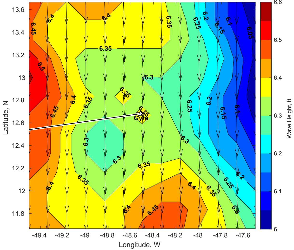
Wave Height (ft) for Gyre at 17-Jan-2025 09:00:00
