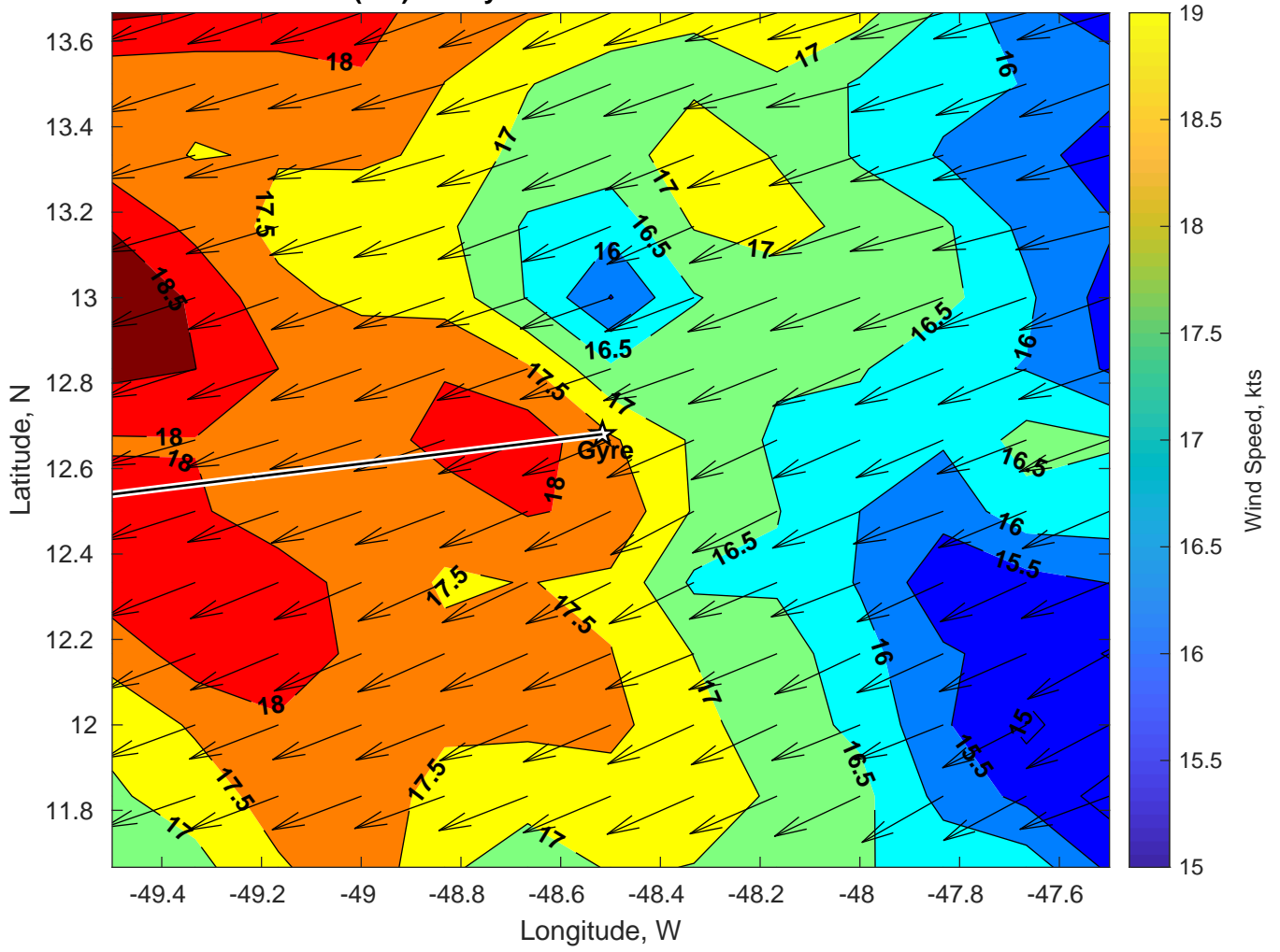
Winds (kts) for Gyre at 17-Jan-2025 09:00:00
