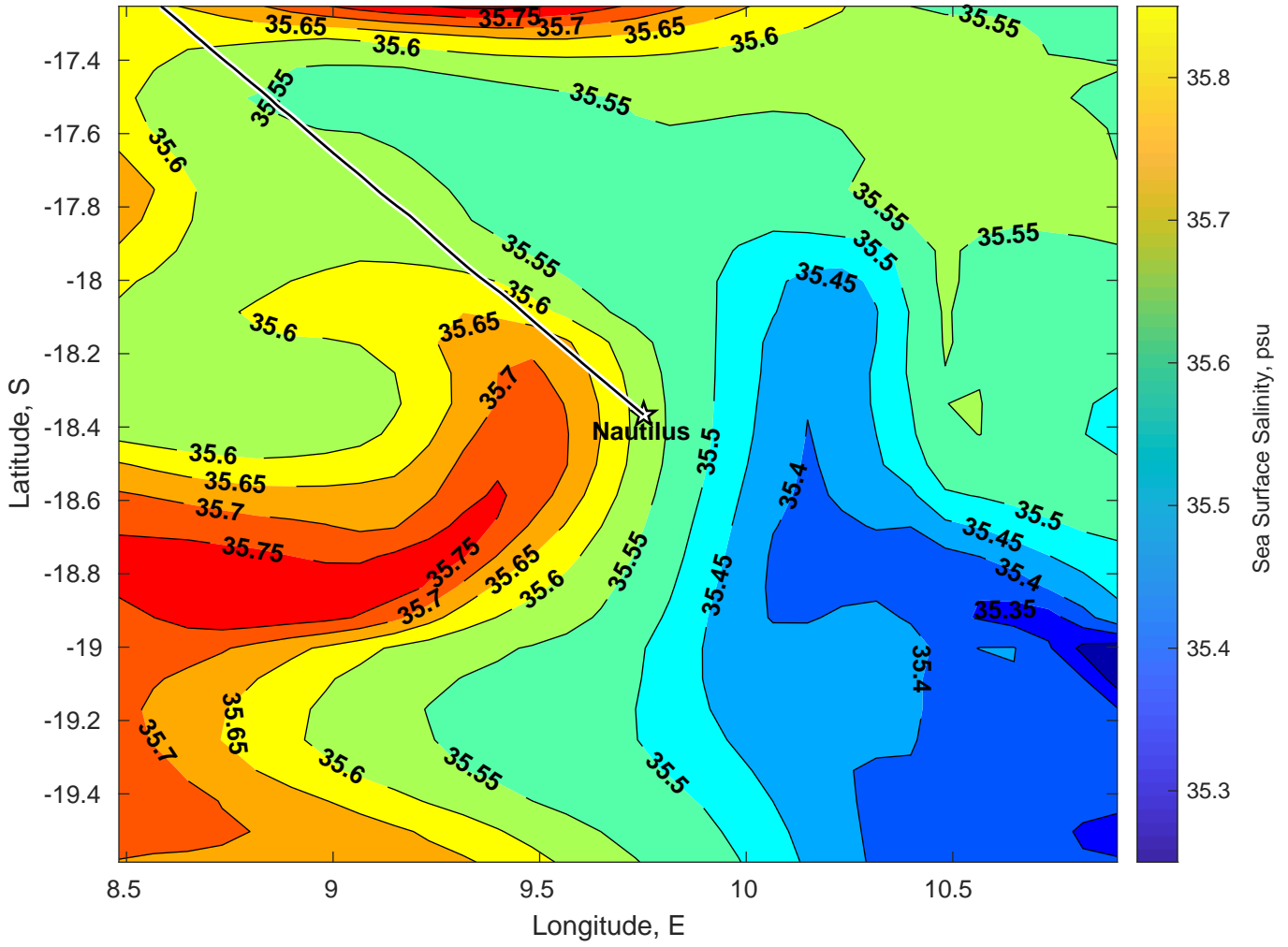
Surface Salinity for Nautilus at 16-Jan-2025 00:00:00
