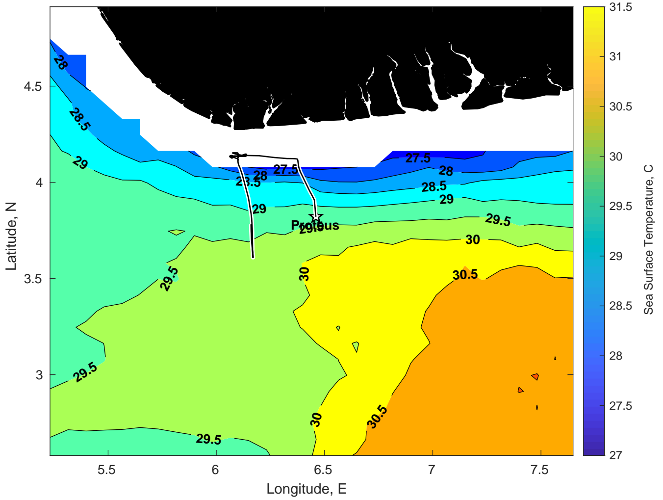
SST for Proteus at 16-Jan-2025 00:00:00
