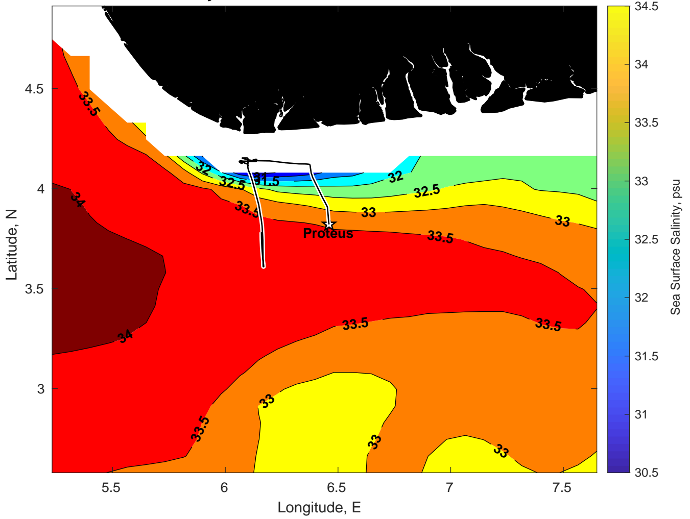
Surface Salinity for Proteus at 16-Jan-2025 00:00:00
