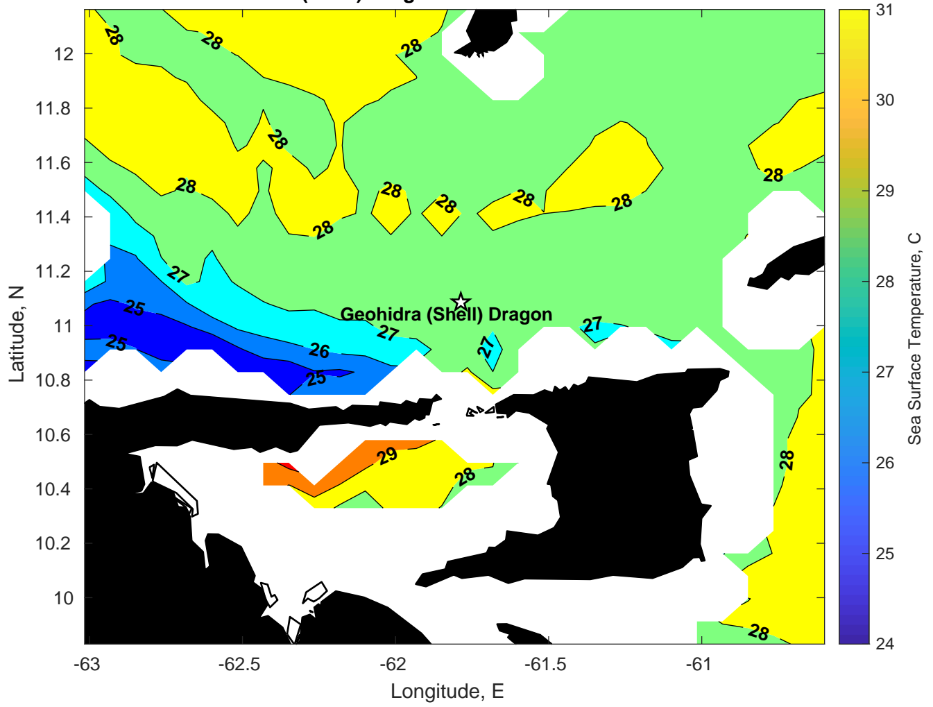
SST for Geohidra (Shell) Dragon at 17-Jan-2025 00:00:00
