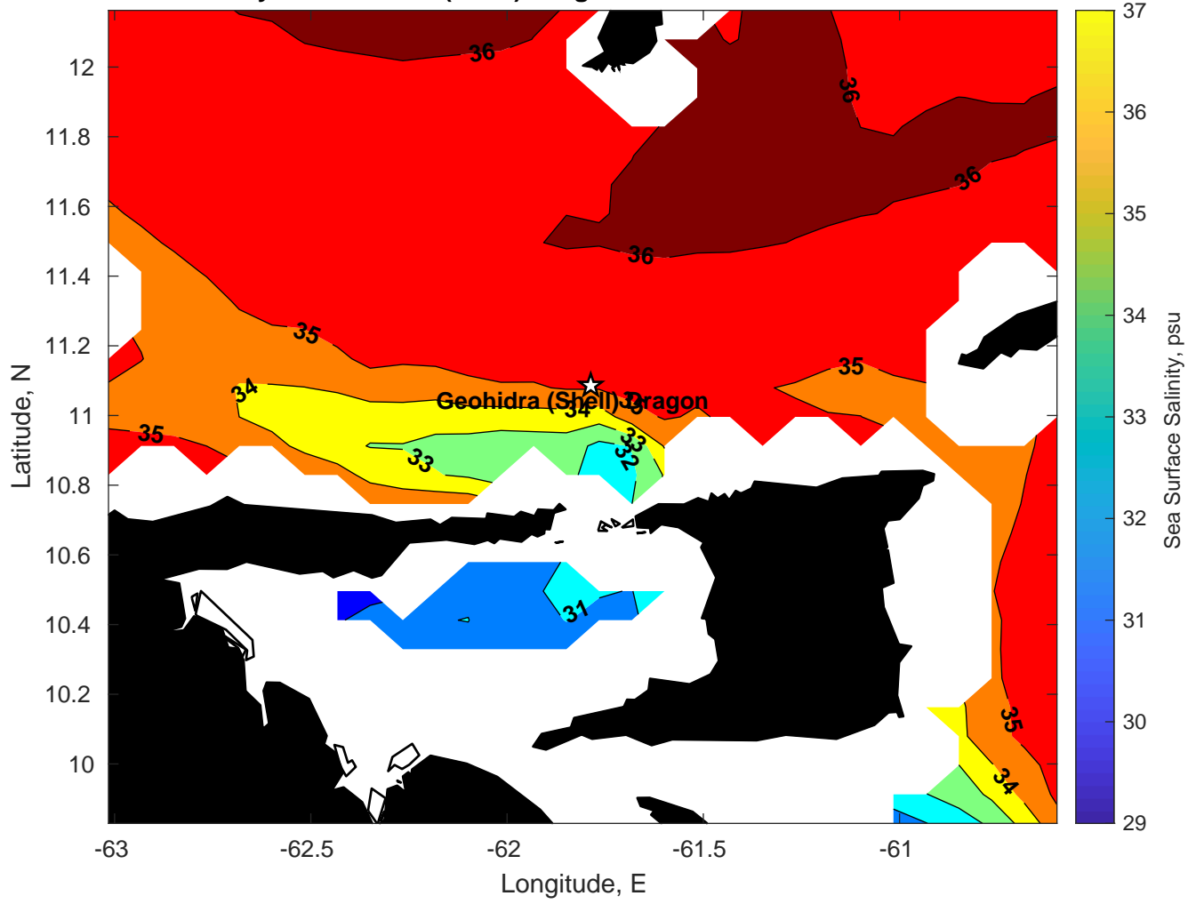
Surface Salinity for Geohidra (Shell) Dragon at 17-Jan-2025 00:00:00
