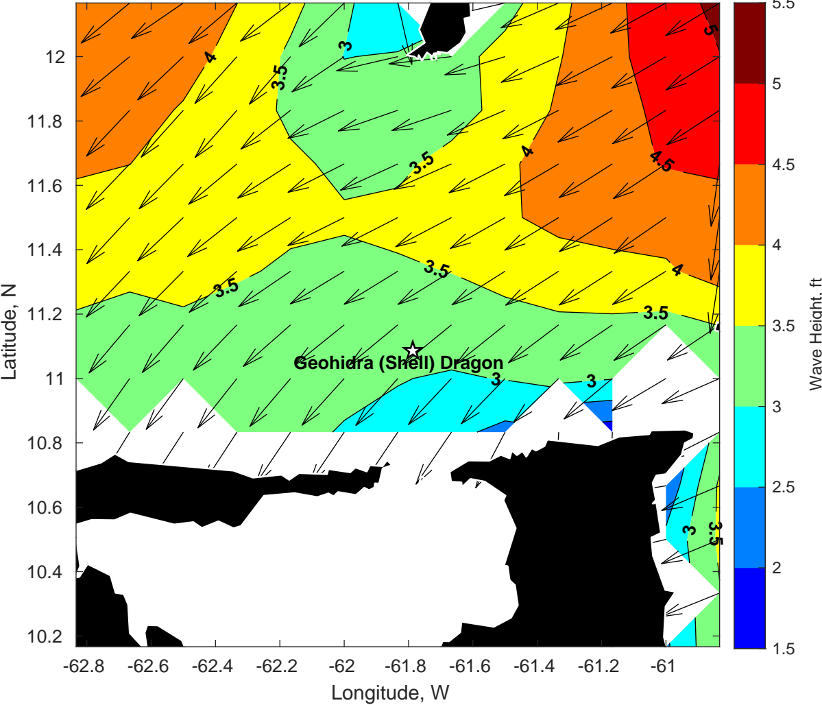
Wave Height (ft) for Geohidra (Shell) Dragon at 18-Jan-2025 09:00:00
