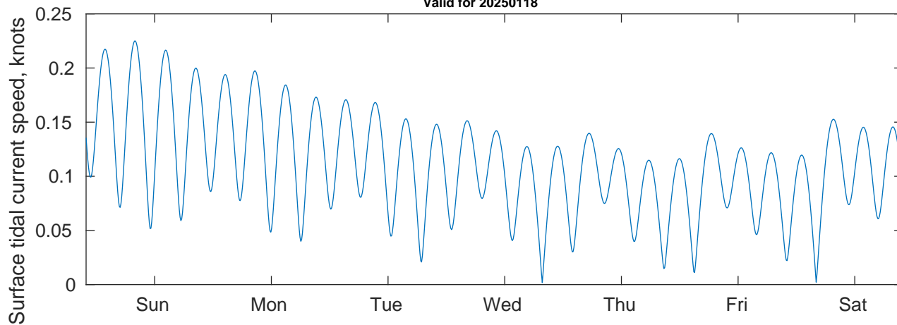
Tidal Currents and Heights for Geohidra (Shell) Dragon at 20250118
