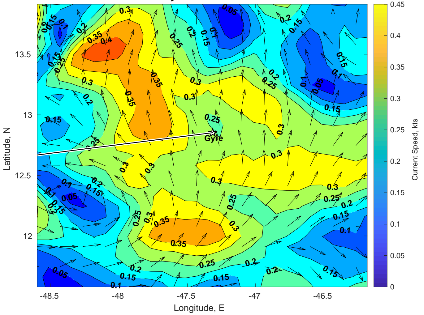
Surface Currents for Gyre at 17-Jan-2025 00:00:00
