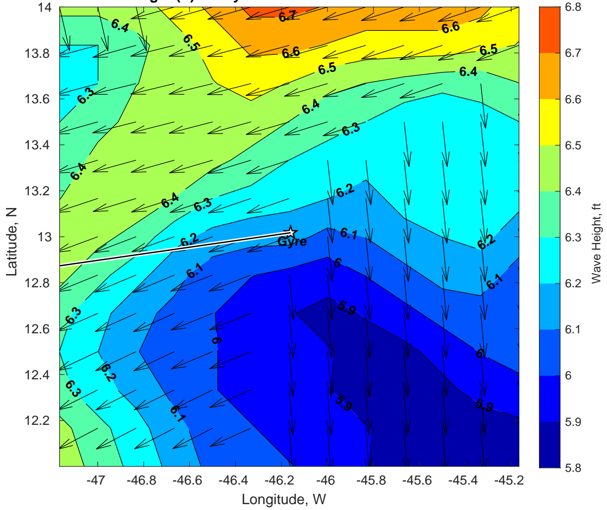
Wave Height (ft) for Gyre at 18-Jan-2025 09:00:00
