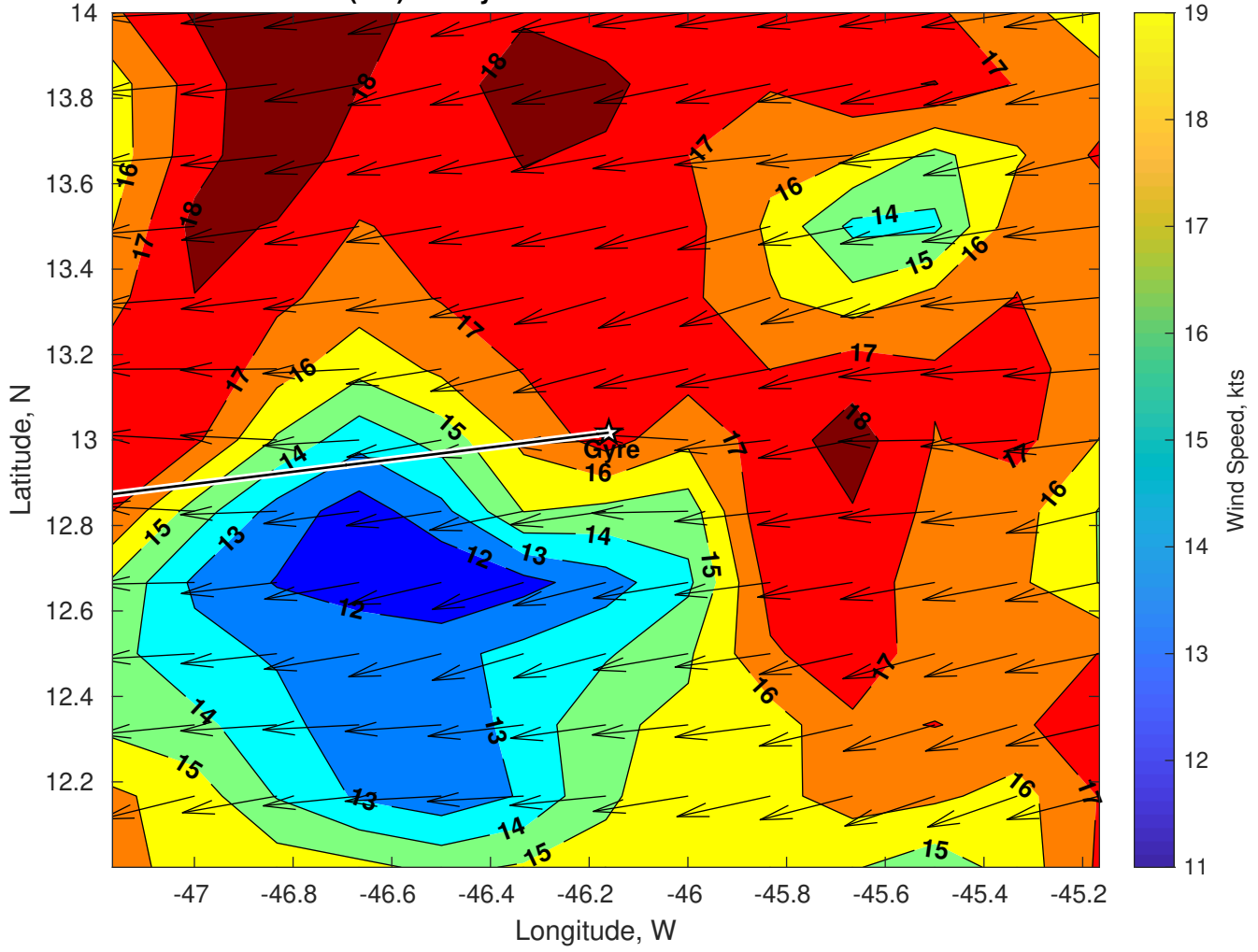
Winds (kts) for Gyre at 18-Jan-2025 09:00:00
