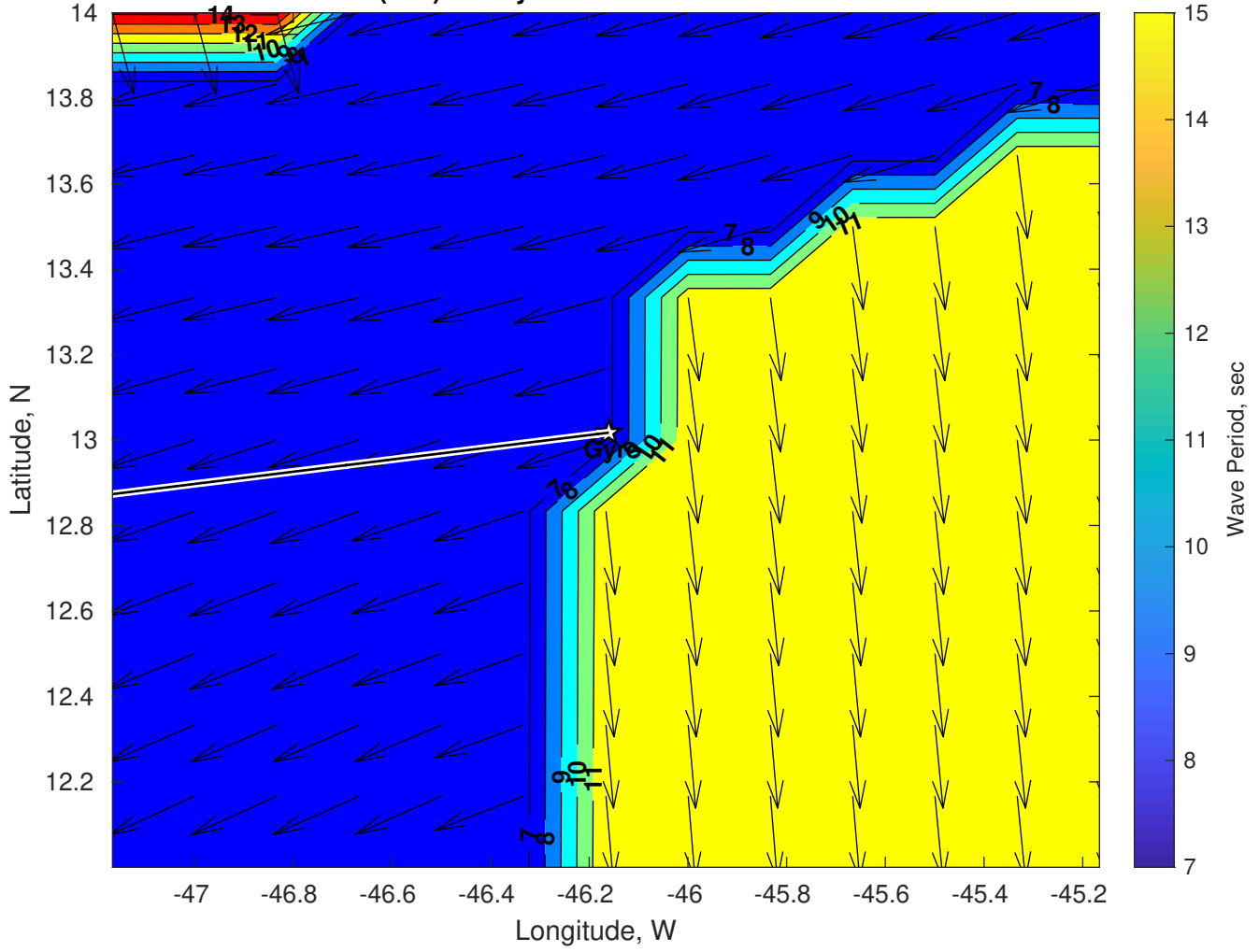
Wave Period (sec) for Gyre at 18-Jan-2025 09:00:00
