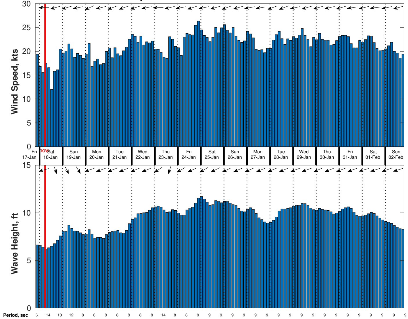
Wind & Wave Forecast for Gyre from 17-Jan-2025 20:00:00 to 02-Feb-2025 20:00:00
