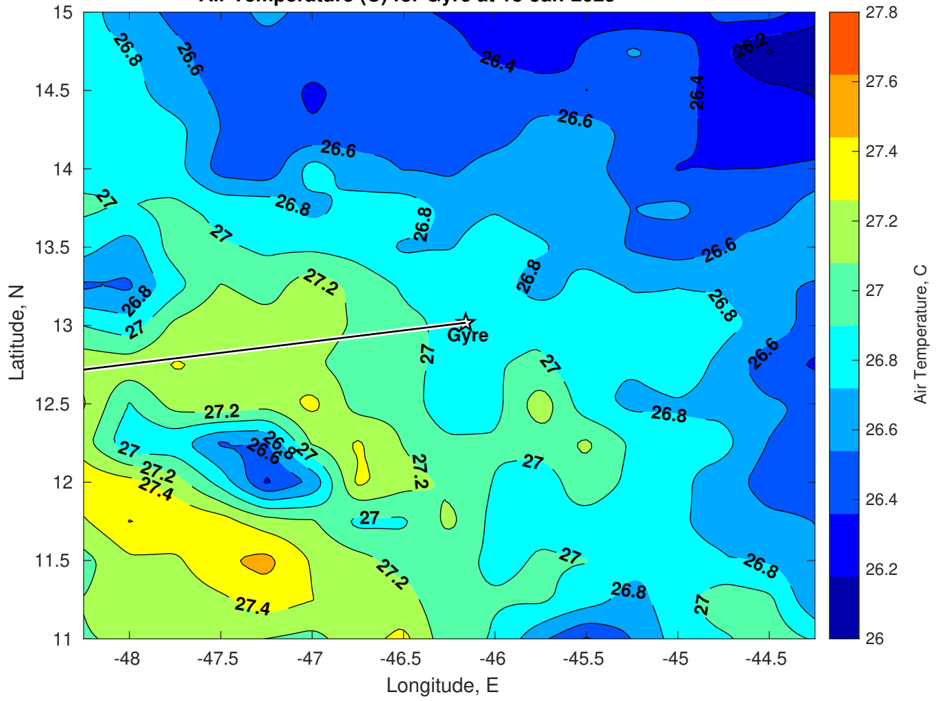
Air Temperature (C) for Gyre at 18-Jan-2025
