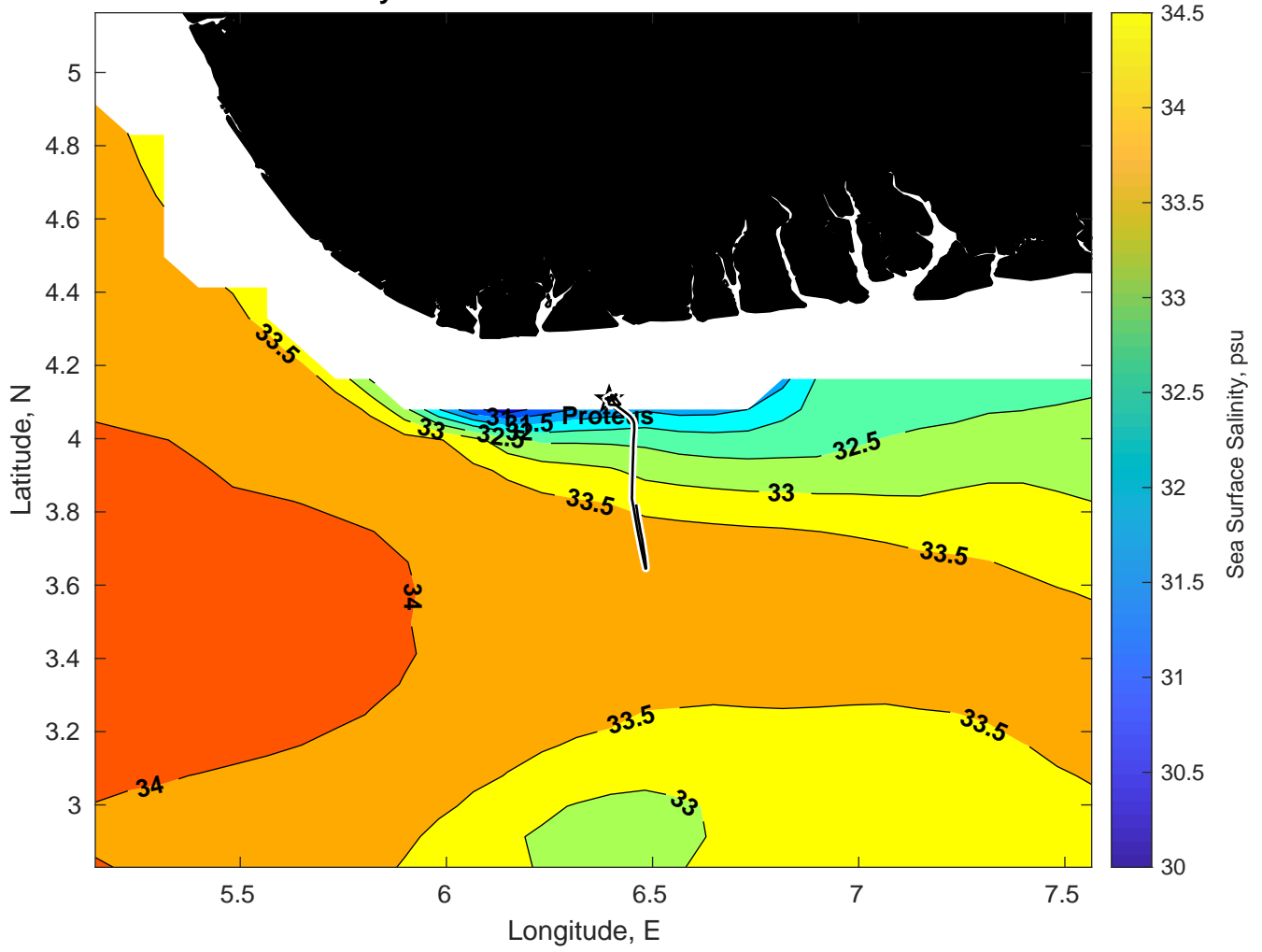
Surface Salinity for Proteus at 17-Jan-2025 00:00:00
