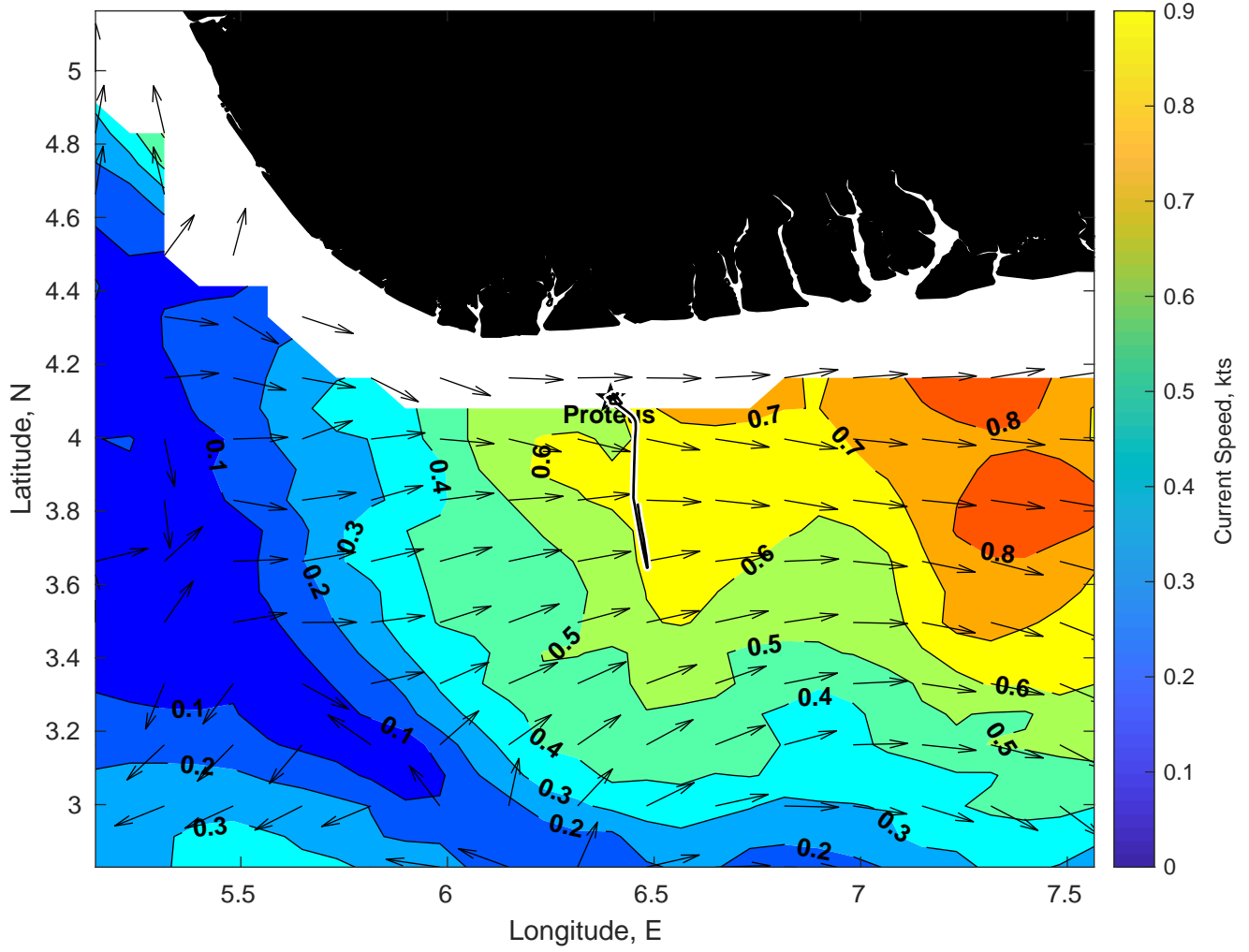
Surface Currents for Proteus at 17-Jan-2025 00:00:00
