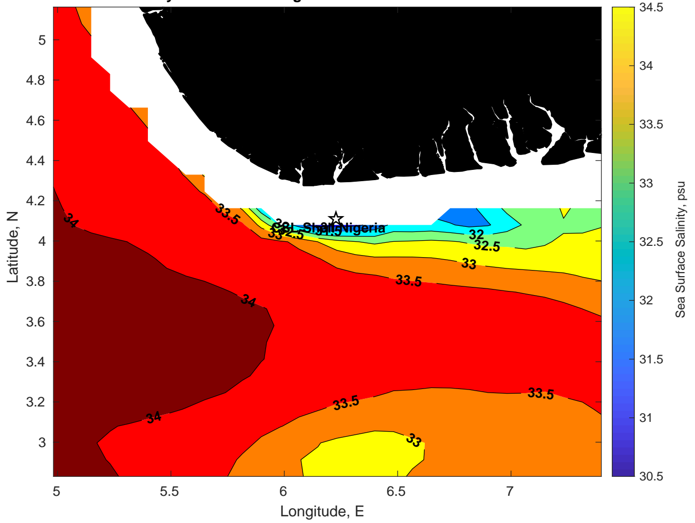
Surface Salinity for CSL Shell Nigeria at 18-Jan-2025 00:00:00
