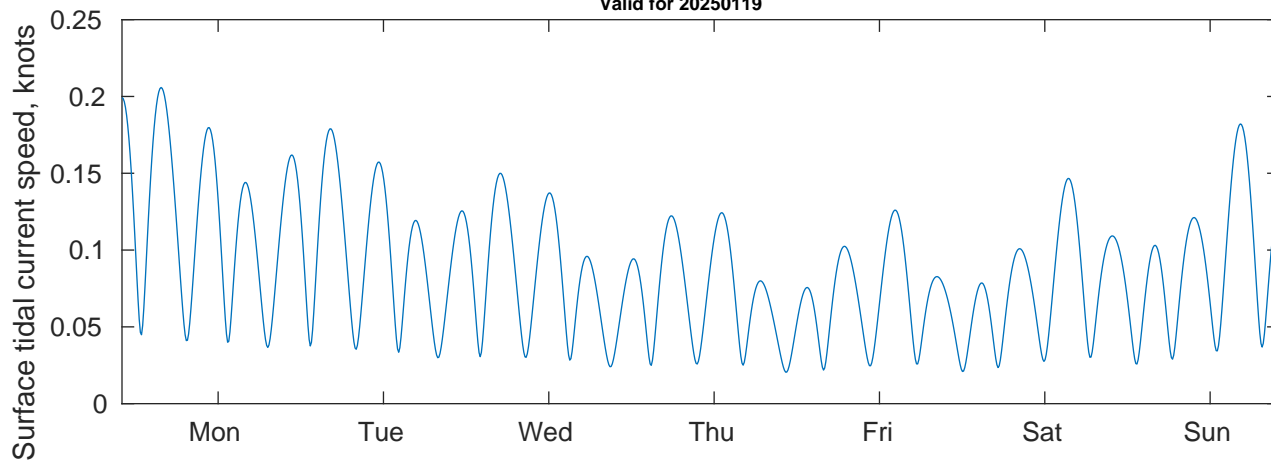
Tidal Currents and Heights for CSL Shell Nigeria at 20250119
