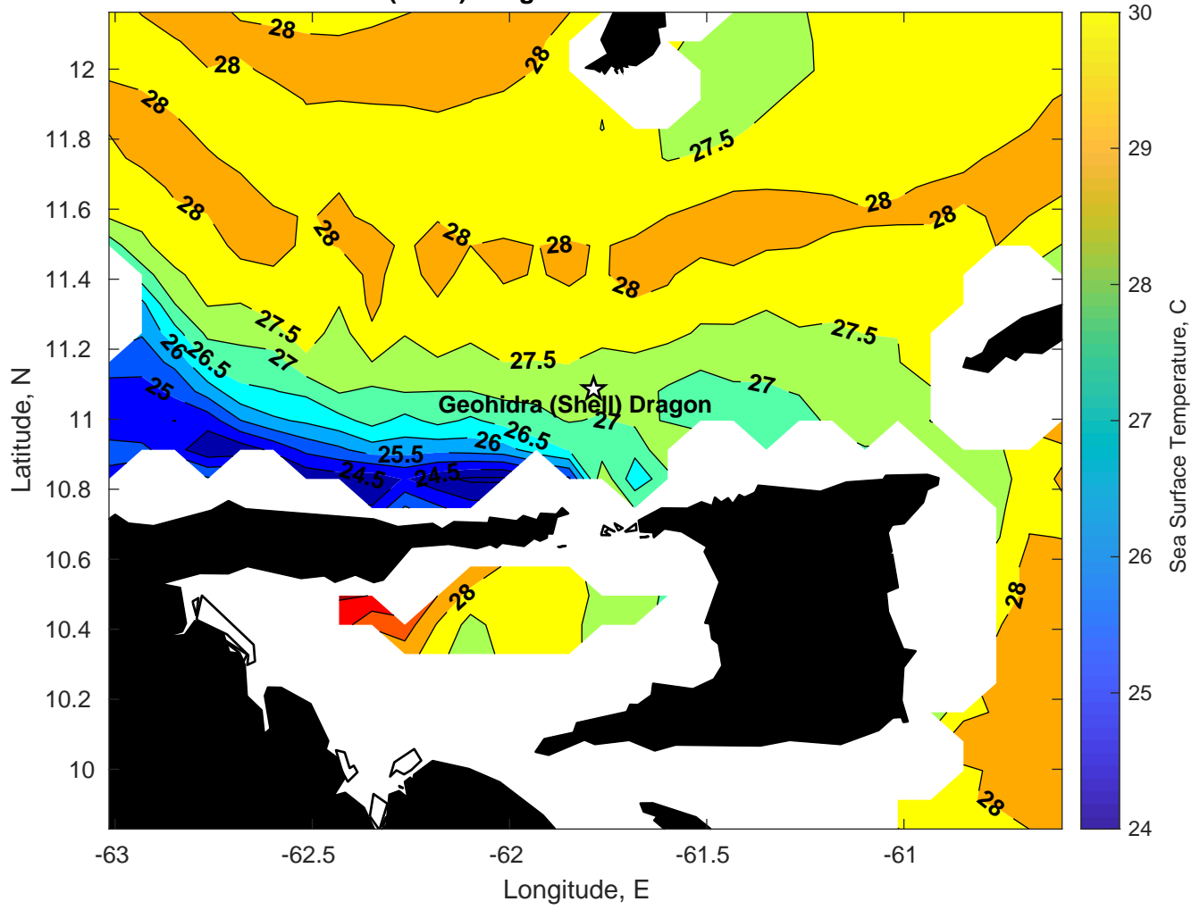
SST for Geohidra (Shell) Dragon at 18-Jan-2025 00:00:00
