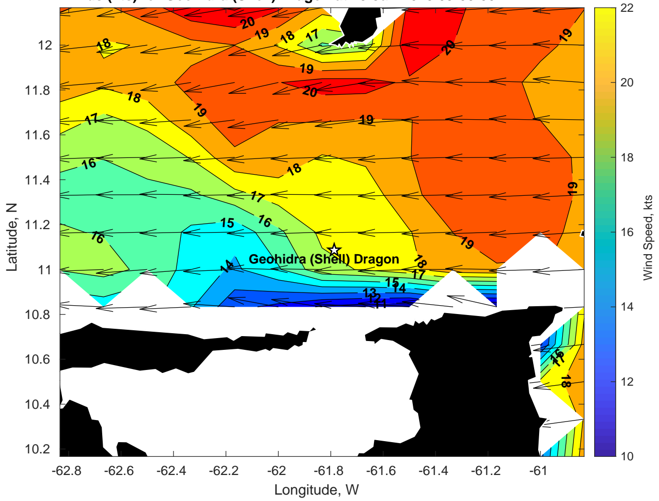
Winds (kts) for Geohidra (Shell) Dragon at 19-Jan-2025 09:00:00
