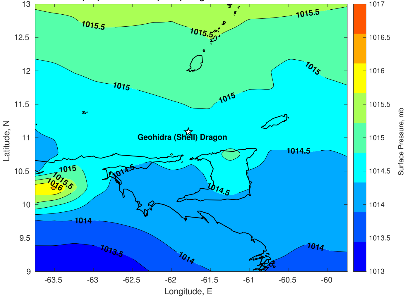
Surface Pressure (mb) for Geohidra (Shell) Dragon at 20-Jan-2025 00:00:00
