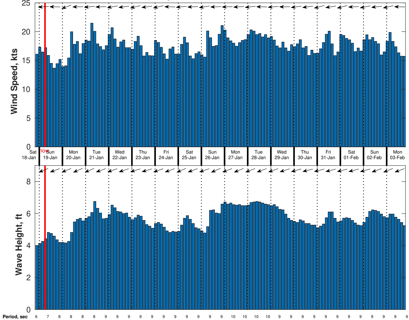
Wind & Wave Forecast for Geohdra (Shell) Dragon from 18-Jan-2025 20:00:00 to 03-Feb-2025 20:00:00
