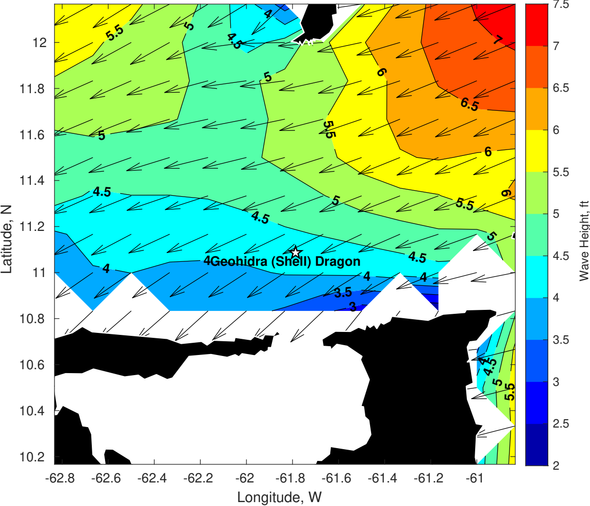
Wave Height (ft) for Geohidra (Shell) Dragon at 19-Jan-2025 09:00:00
