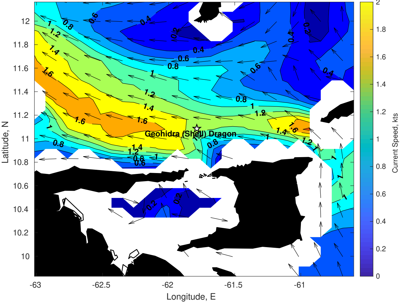
Surface Currents for Geohidra (Shell) Dragon at 18-Jan-2025 00:00:00
