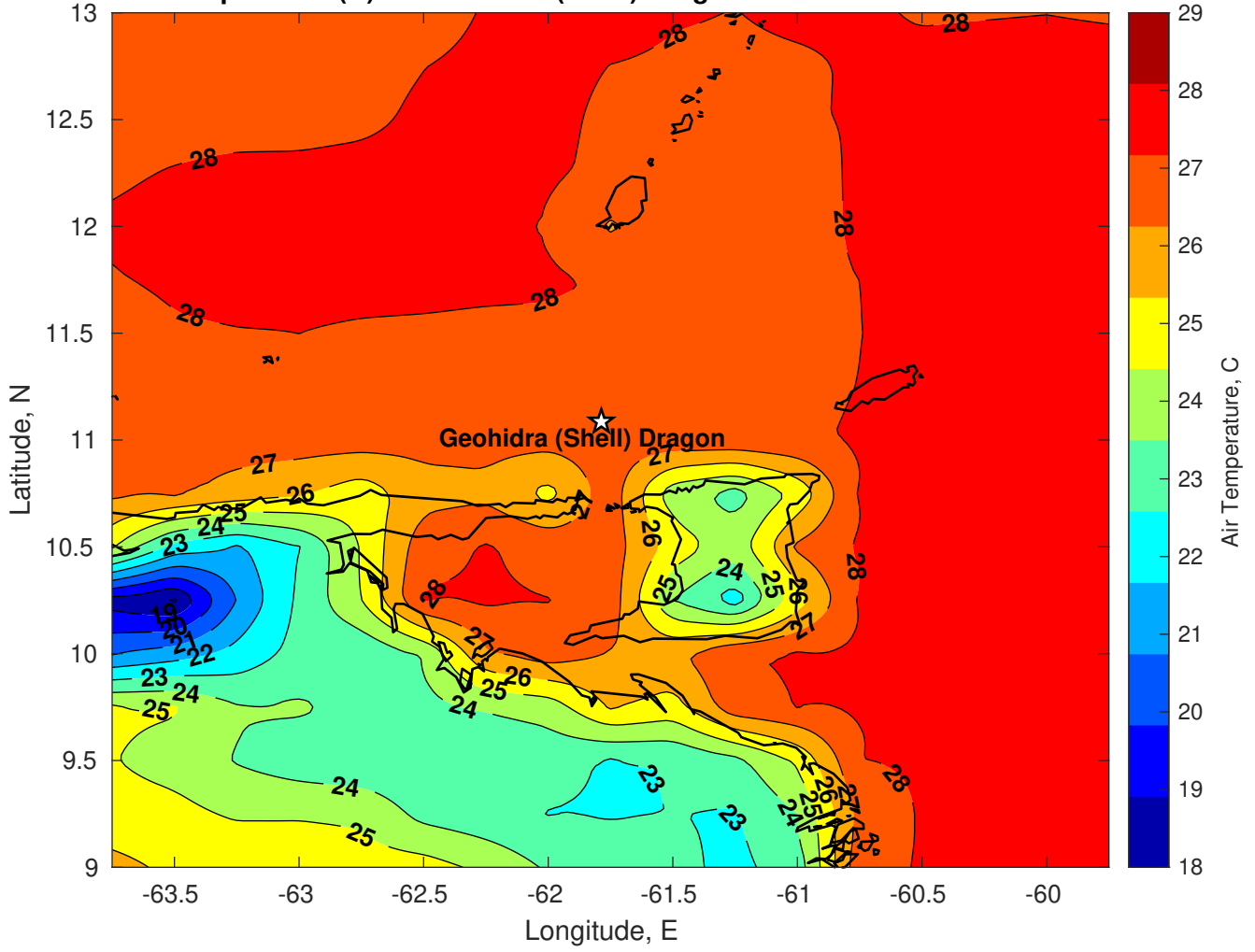
Air Temperature (C) for Geohidra (Shell) Dragon at 19-Jan-2025
