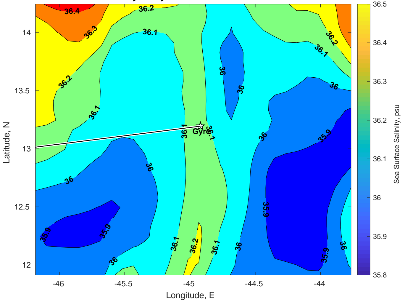
Surface Salinity for Gyre at 18-Jan-2025 00:00:00
