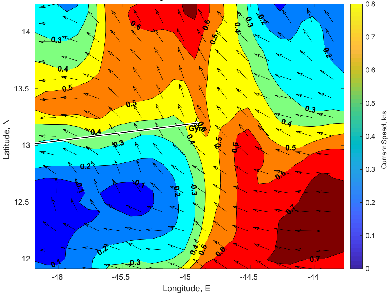
Surface Currents for Gyre at 18-Jan-2025 00:00:00
