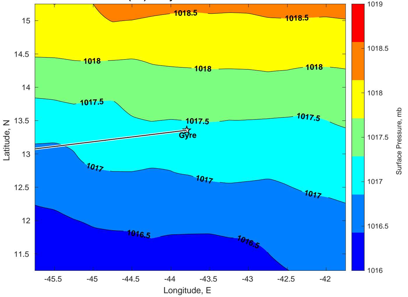
Surface Pressure (mb) for Gyre at 20-Jan-2025 00:00:00
