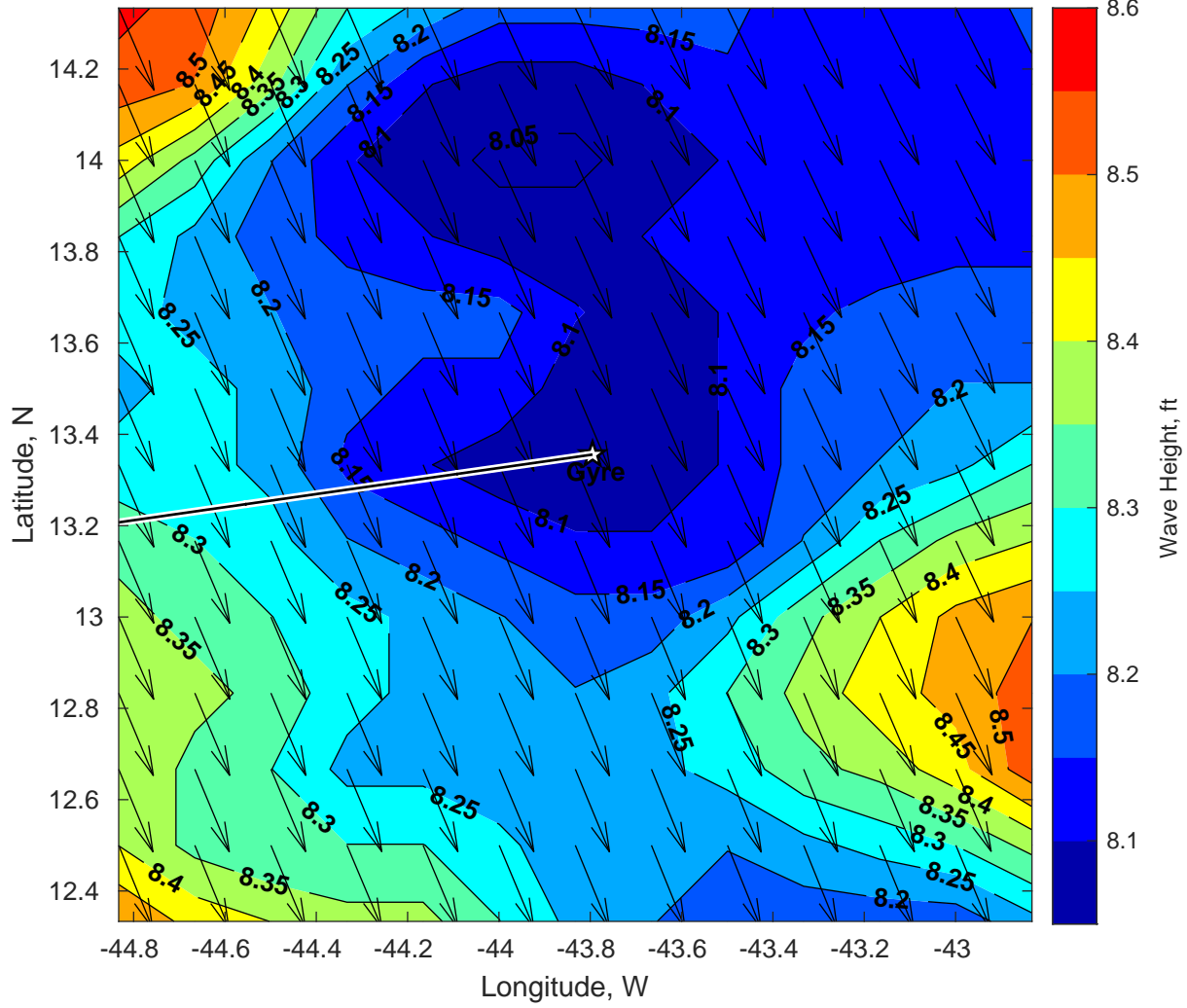
Wave Height (ft) for Gyre at 19-Jan-2025 09:00:00
