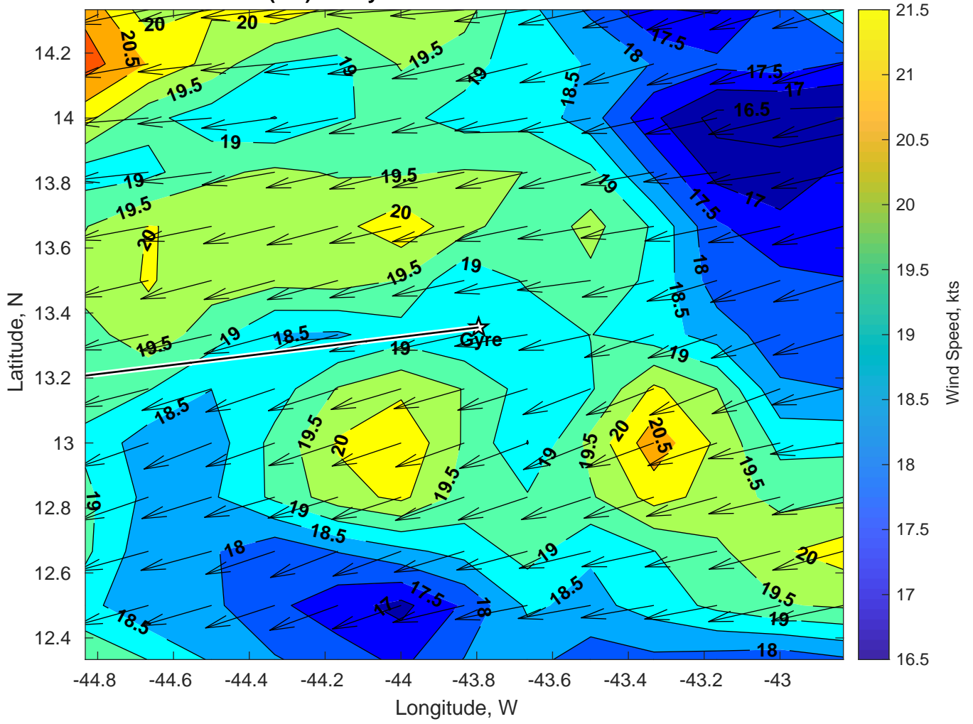
Winds (kts) for Gyre at 19-Jan-2025 09:00:00
