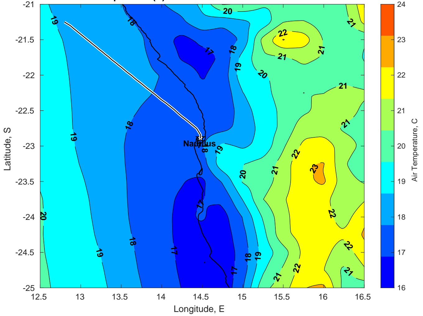
Air Temperature (C) for Nautilus at 19-Jan-2025
