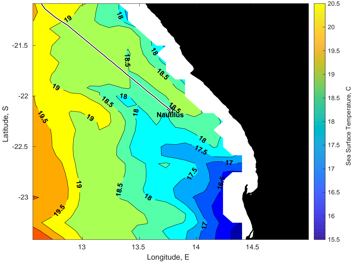
SST for Nautilus at 18-Jan-2025 00:00:00
