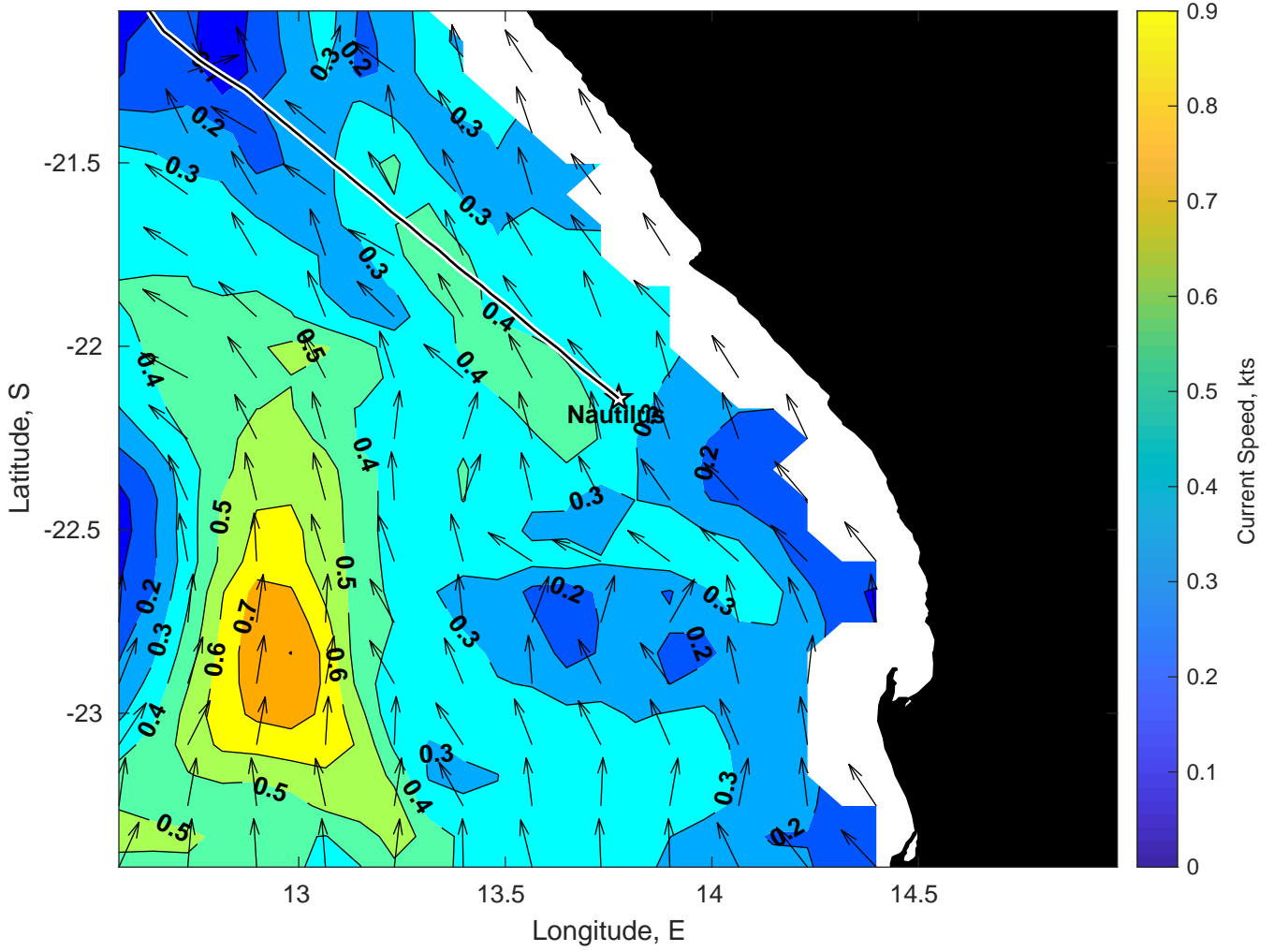
Surface Currents for Nautilus at 18-Jan-2025 00:00:00
