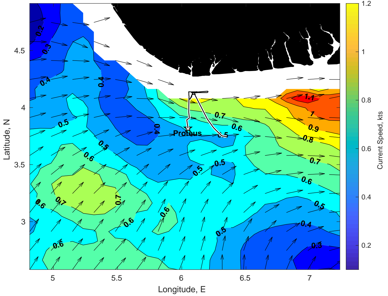
Surface Currents for Proteus at 18-Jan-2025 00:00:00
