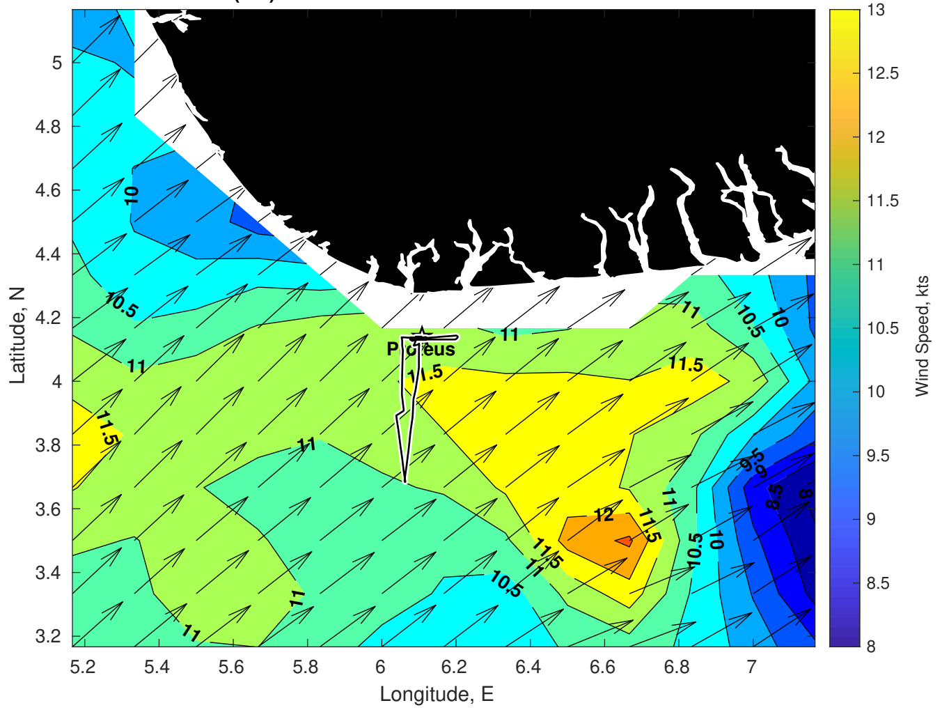
Winds (kts) for Proteus at 19-Jan-2025 09:00:00
