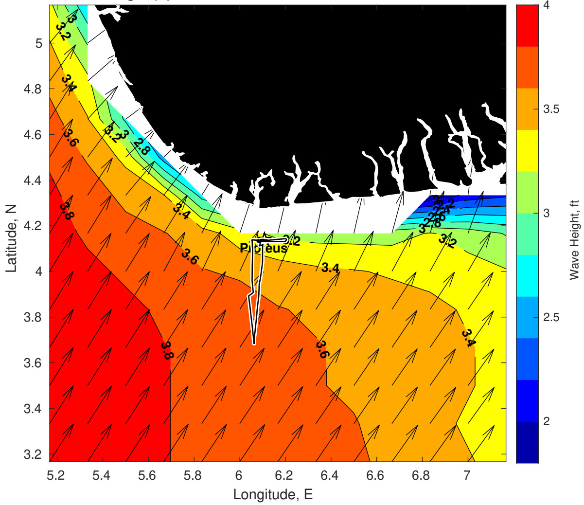
Wave Height (ft) for Proteus at 19-Jan-2025 09:00:00
