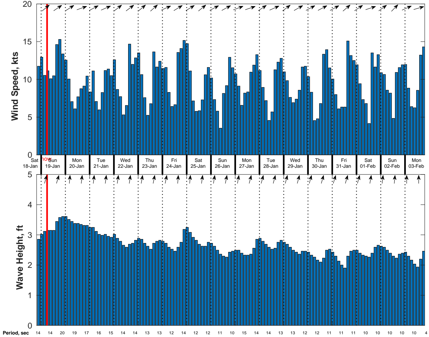
Wind & Wave Forecast for Proteus from 18-Jan-2025 20:00:00 to 03-Feb-2025 20:00:00
