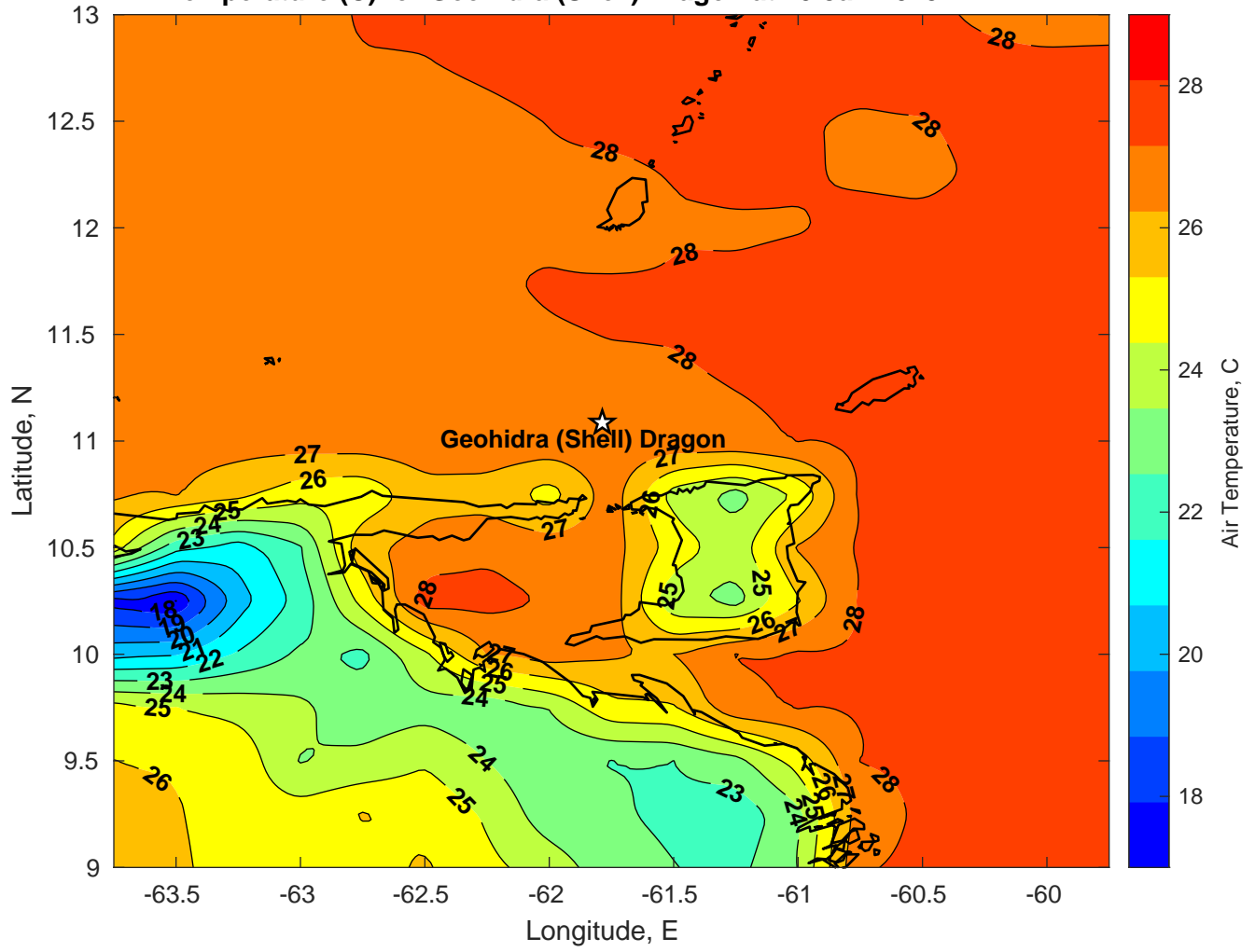
Air Temperature (C) for Geohidra (Shell) Dragon at 20-Jan-2025
