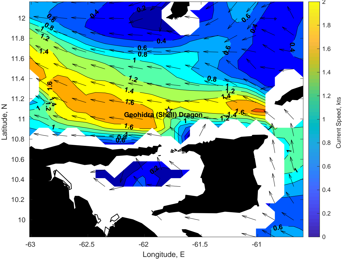
Surface Currents for Geohidra (Shell) Dragon at 19-Jan-2025 00:00:00
