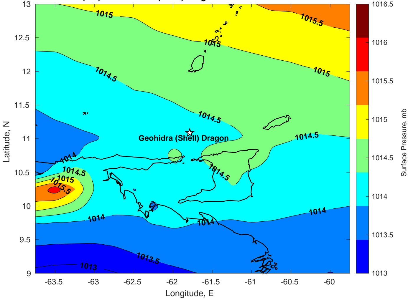
Surface Pressure (mb) for Geohidra (Shell) Dragon at 22-Jan-2025 00:00:00
