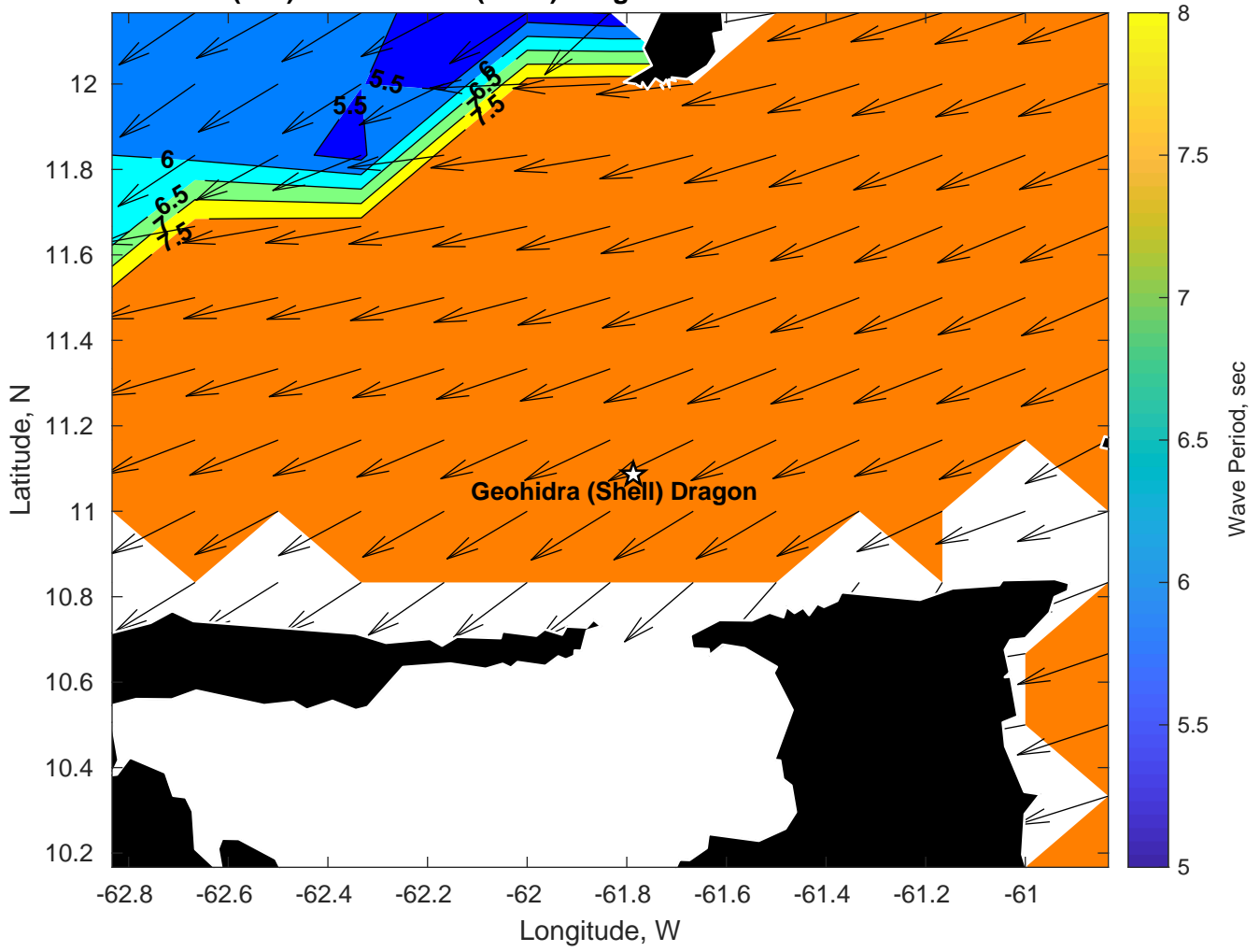
Wave Period (sec) for Geohidra (Shell) Dragon at 20-Jan-2025 09:00:00
