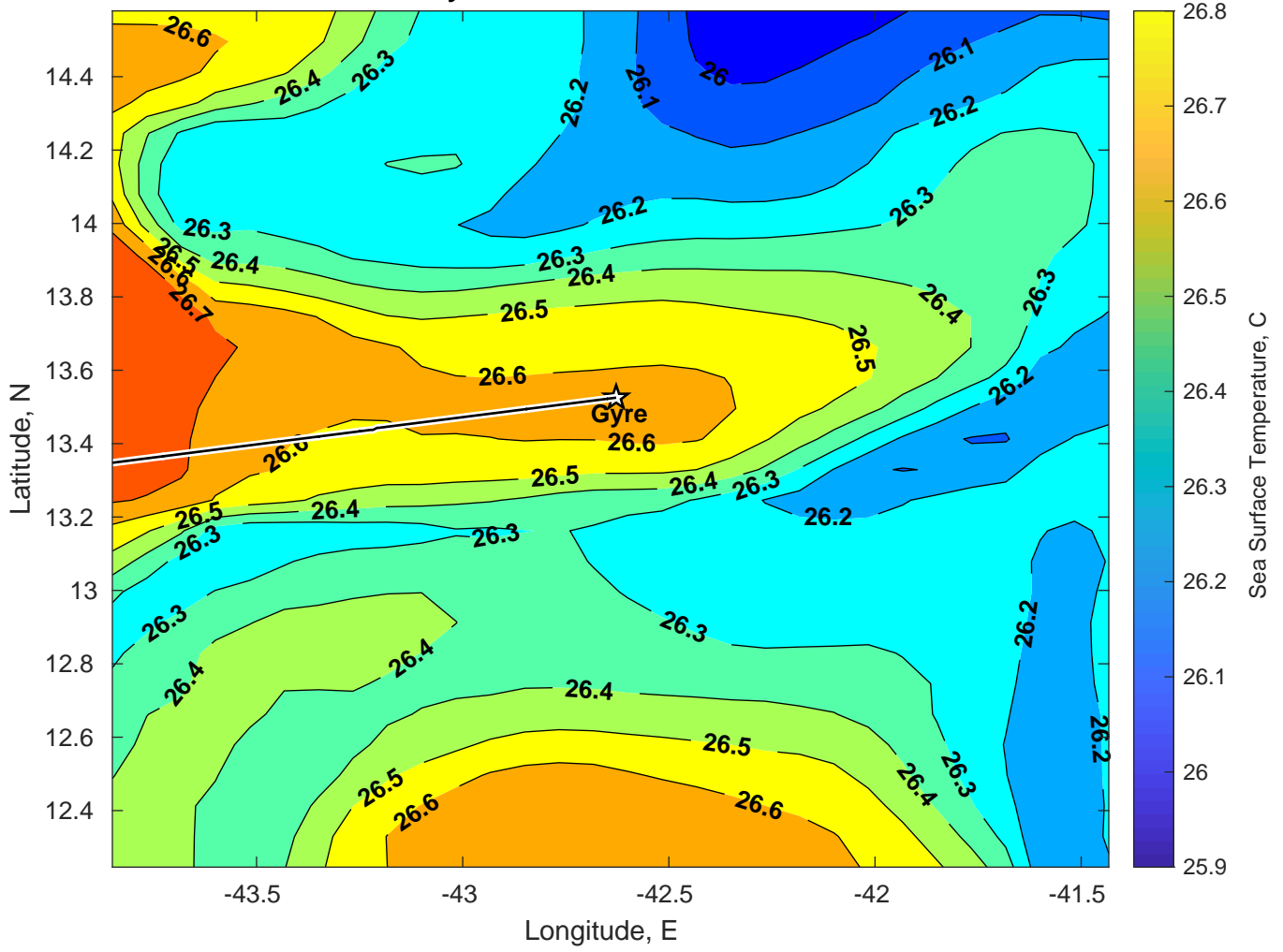
SST for Gyre at 19-Jan-2025 00:00:00
