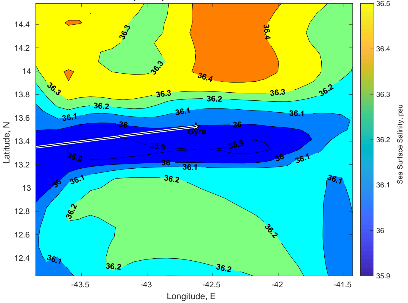
Surface Salinity for Gyre at 19-Jan-2025 00:00:00
