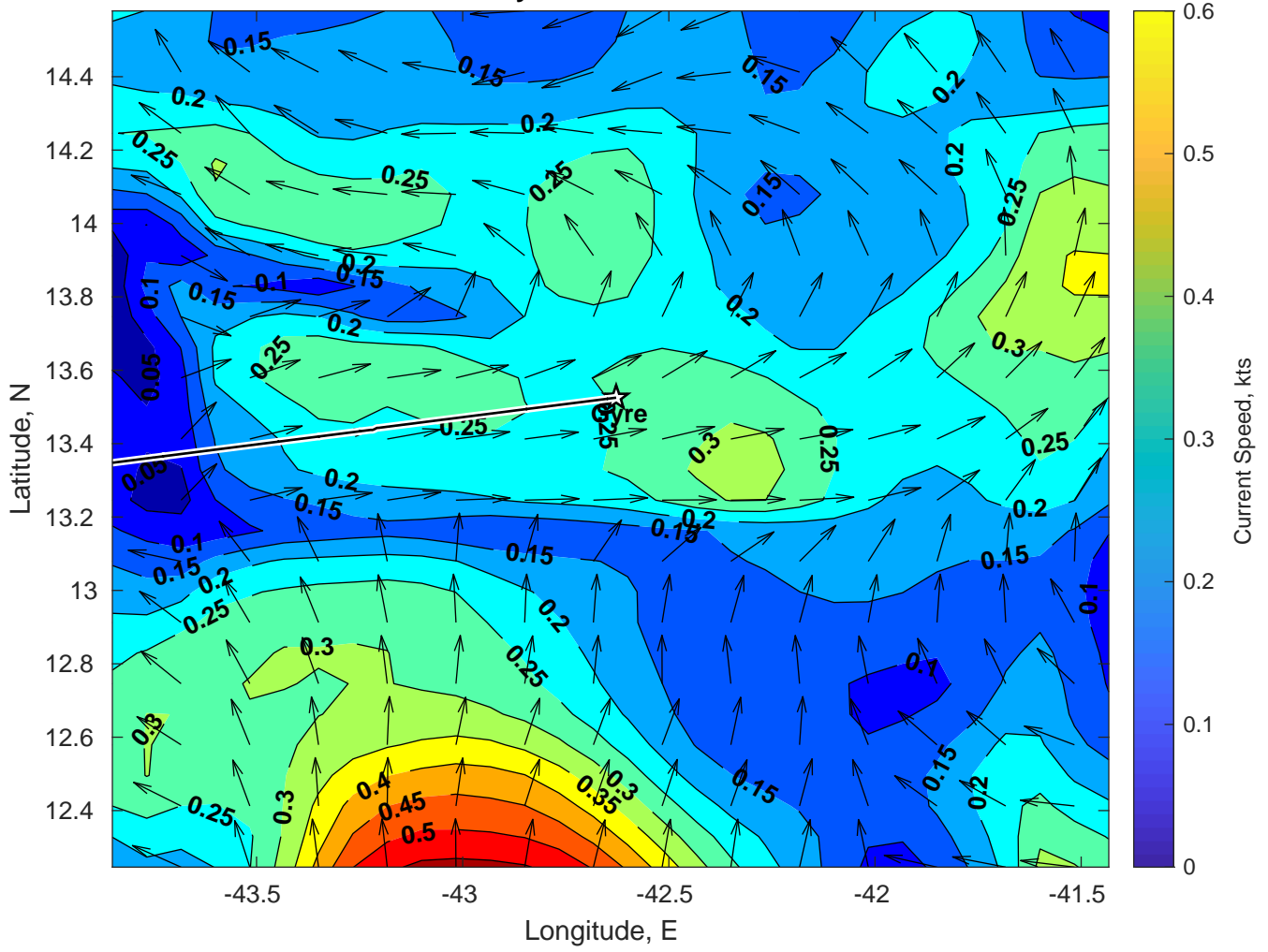
Surface Currents for Gyre at 19-Jan-2025 00:00:00
