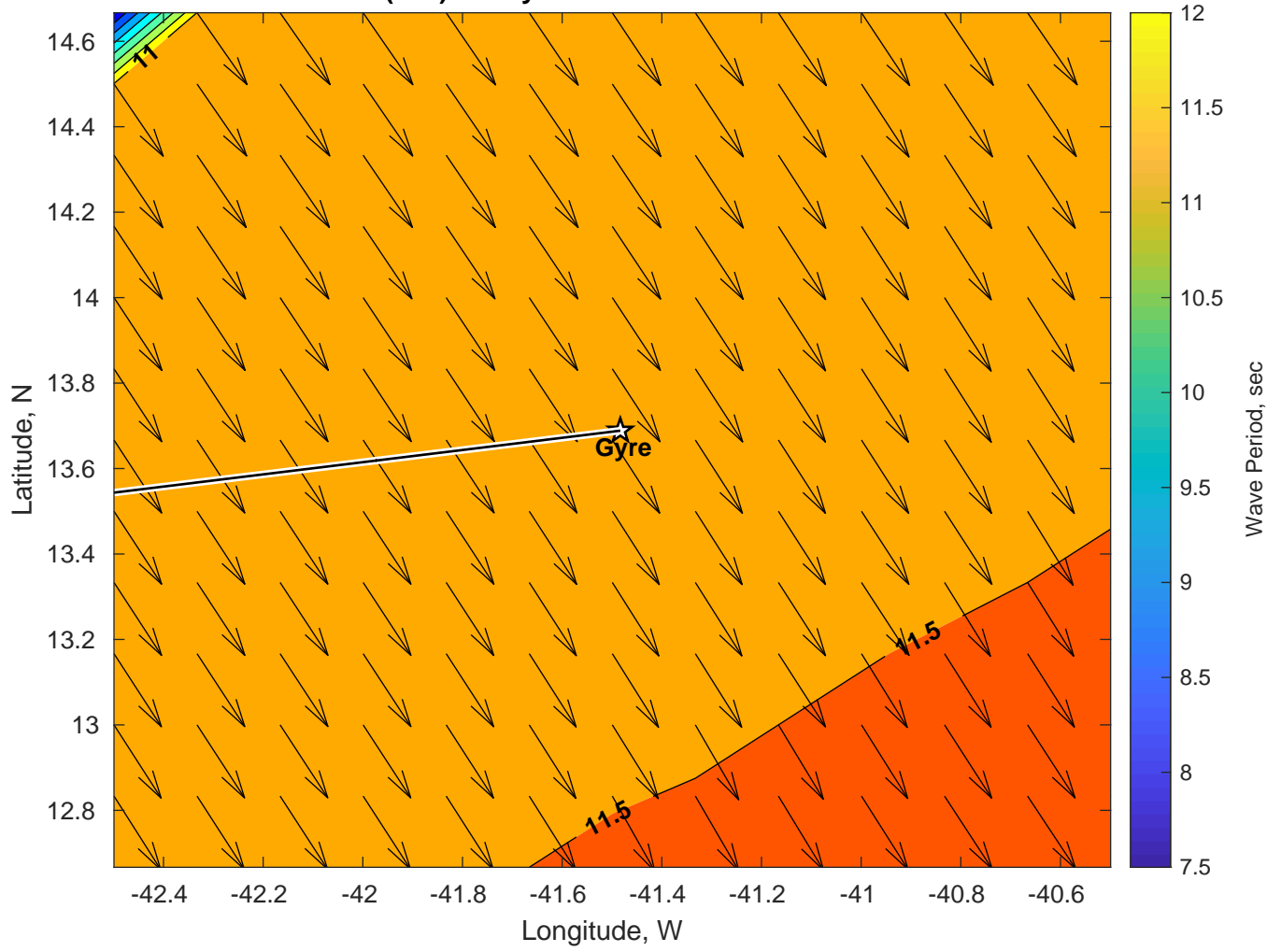
Wave Period (sec) for Gyre at 20-Jan-2025 09:00:00
