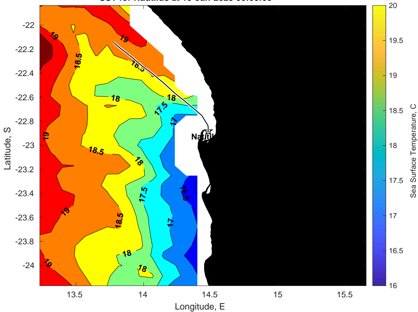
SST for Nautilus at 19-Jan-2025 00:00:00
