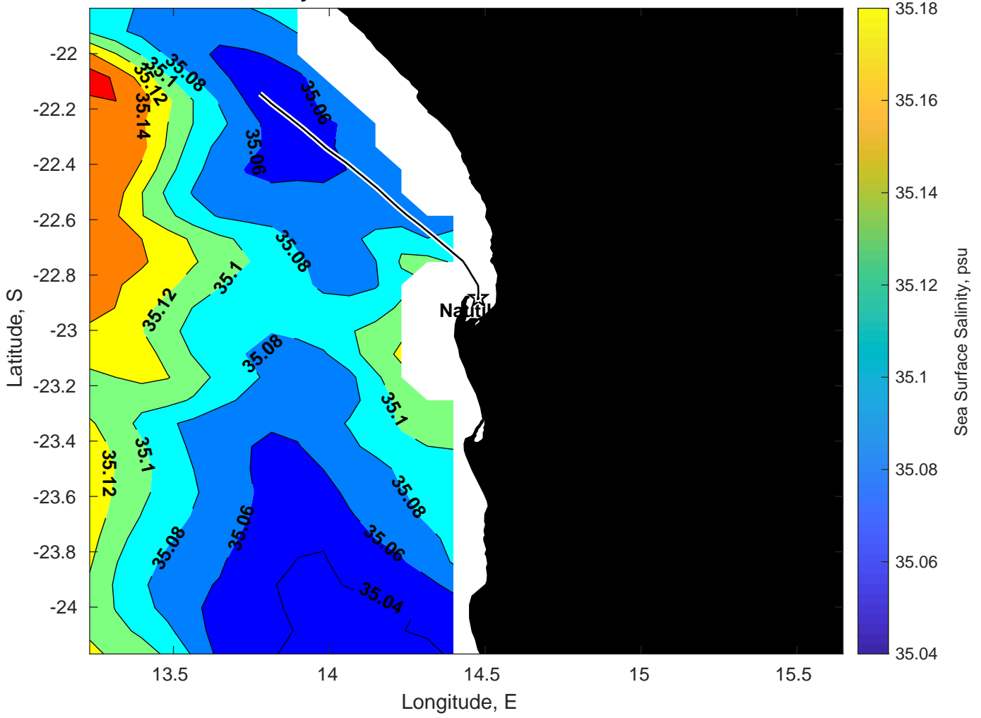
Surface Salinity for Nautilus at 19-Jan-2025 00:00:00
