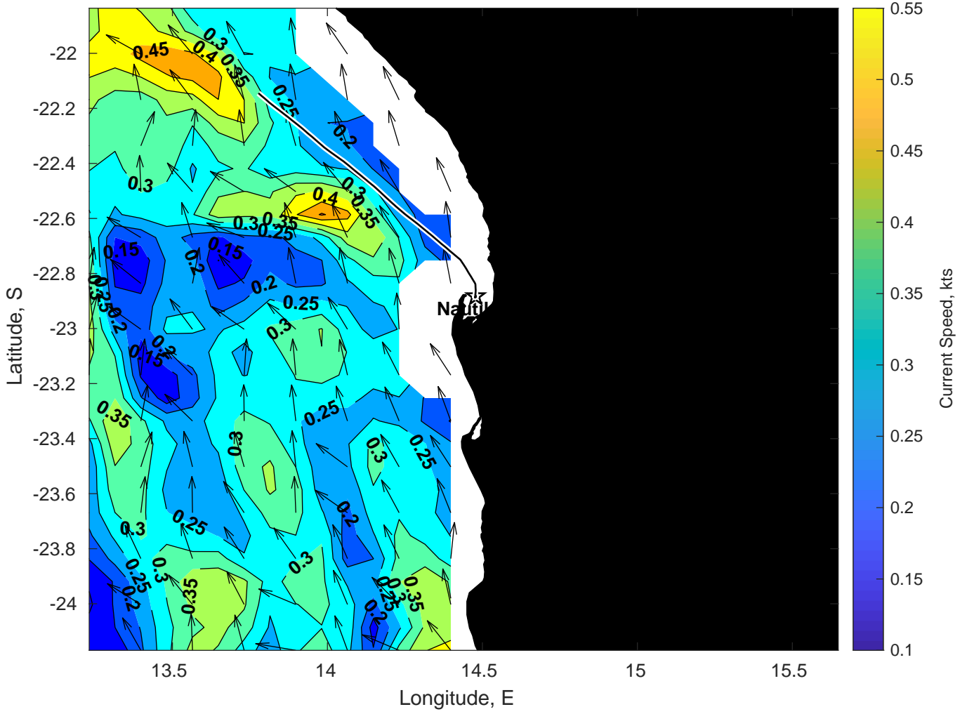
Surface Currents for Nautilus at 19-Jan-2025 00:00:00
