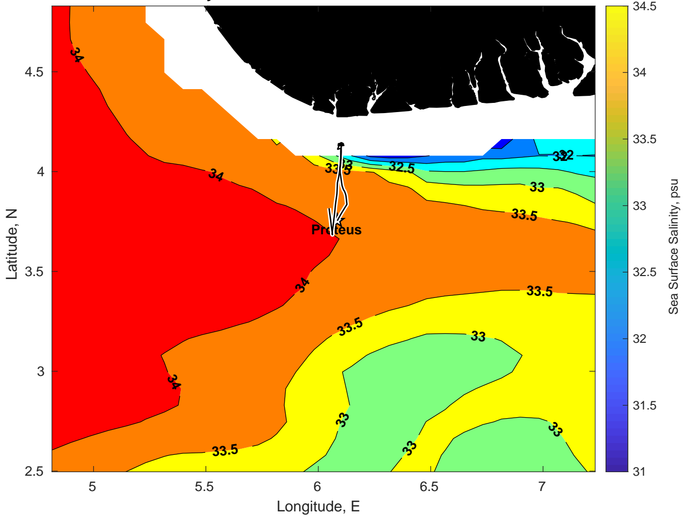
Surface Salinity for Proteus at 19-Jan-2025 00:00:00
