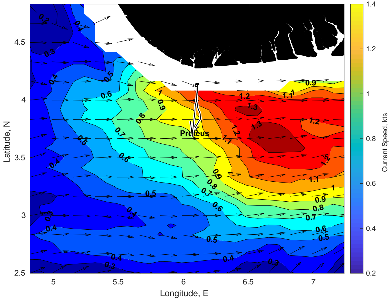
Surface Currents for Proteus at 19-Jan-2025 00:00:00
