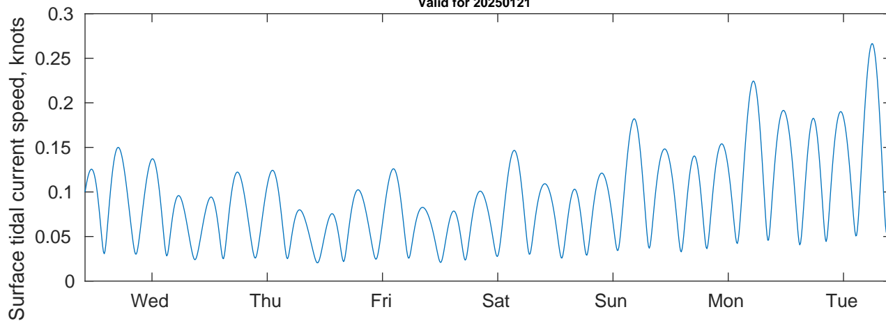
Tidal Currents and Heights for CSL Shell Nigeria at 20250121
