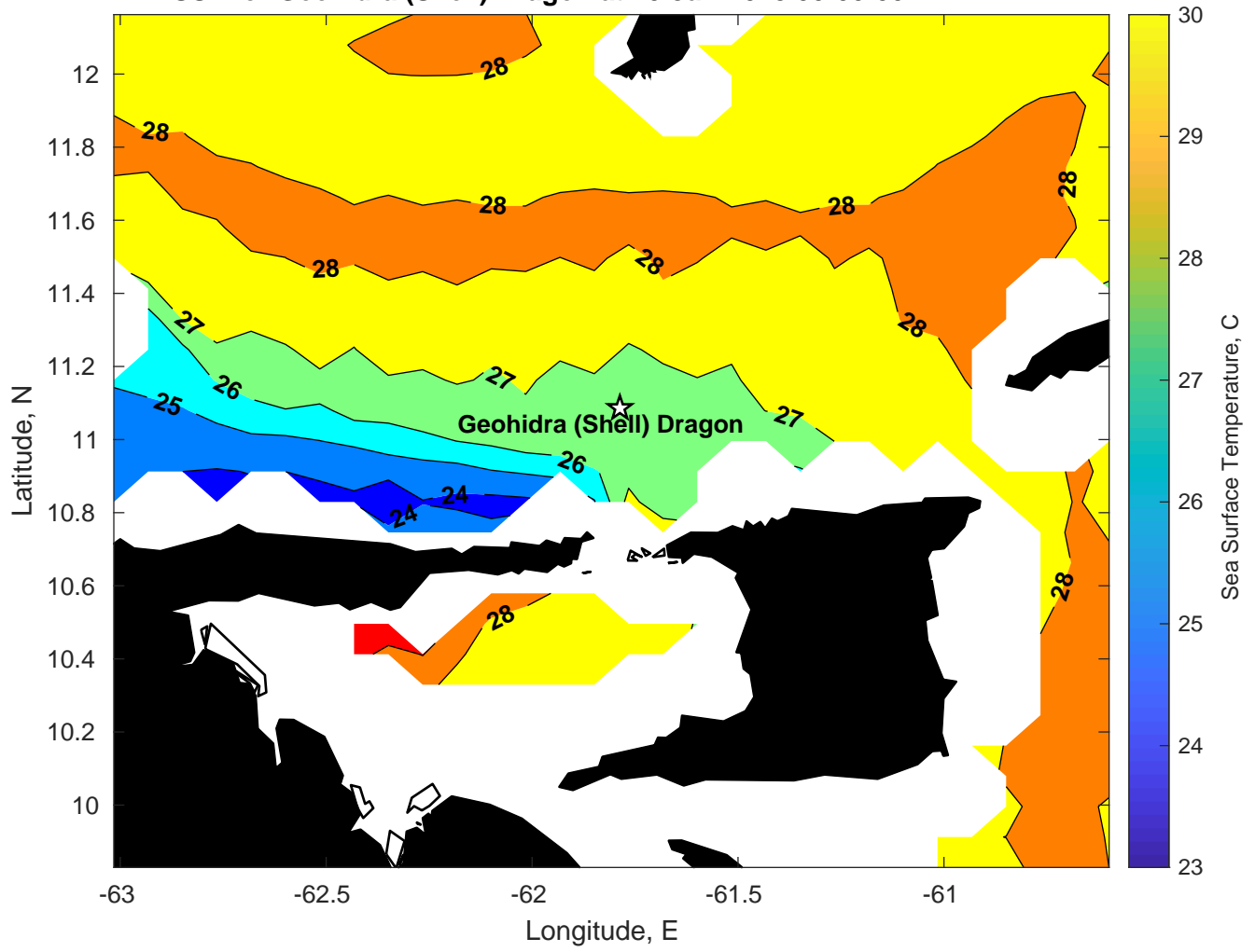
SST for Geohidra (Shell) Dragon at 20-Jan-2025 00:00:00
