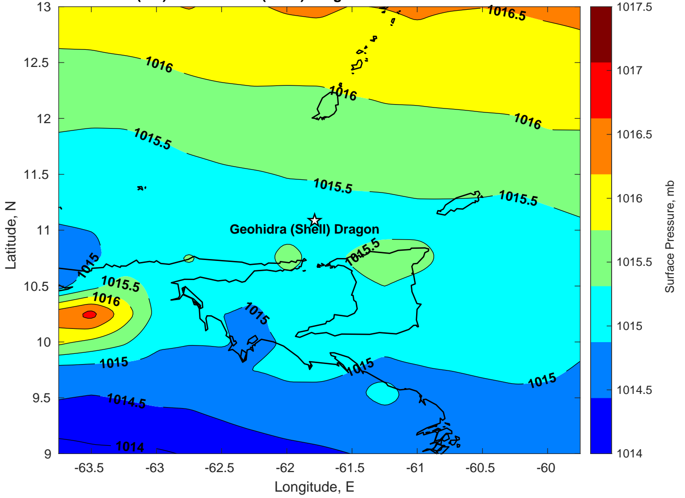
Surface Pressure (mb) for Geohidra (Shell) Dragon at 23-Jan-2025 00:00:00
