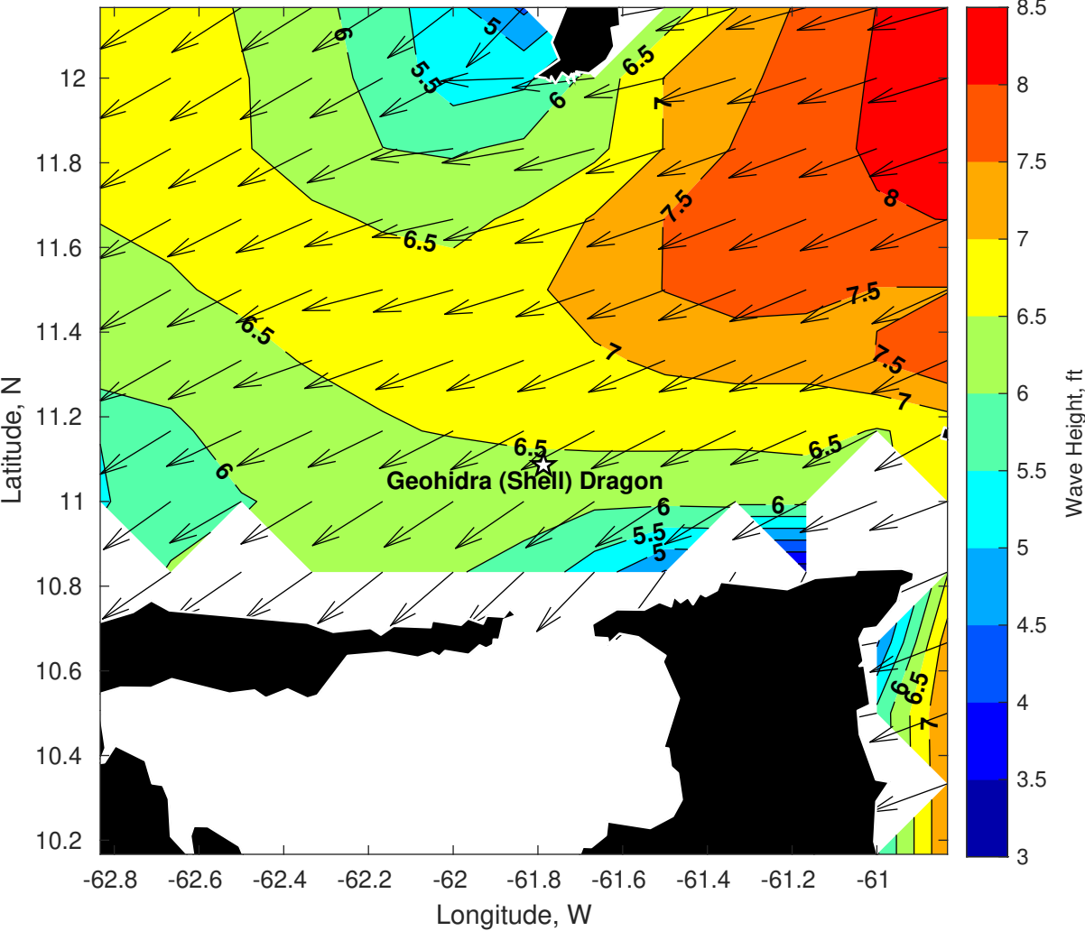
Wave Height (ft) for Geohidra (Shell) Dragon at 21-Jan-2025 09:00:00
