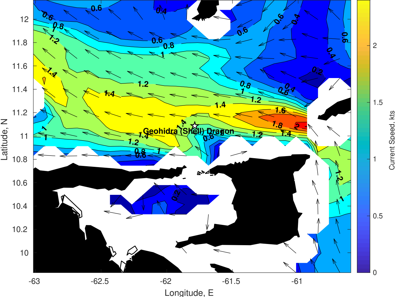
Surface Currents for Geohidra (Shell) Dragon at 20-Jan-2025 00:00:00
