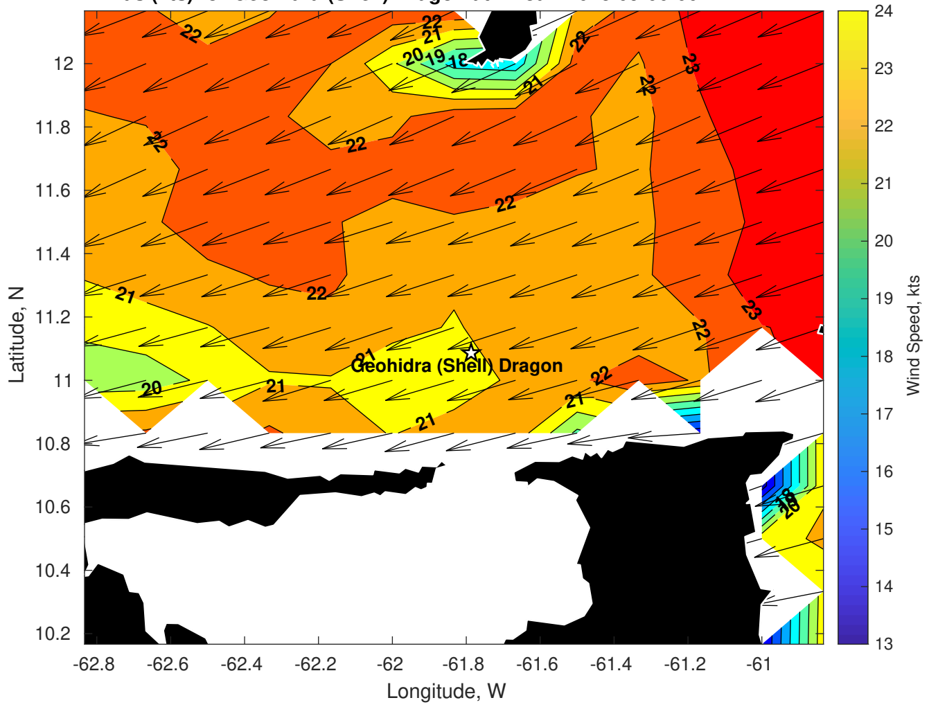
Winds (kts) for Geohidra (Shell) Dragon at 21-Jan-2025 09:00:00
