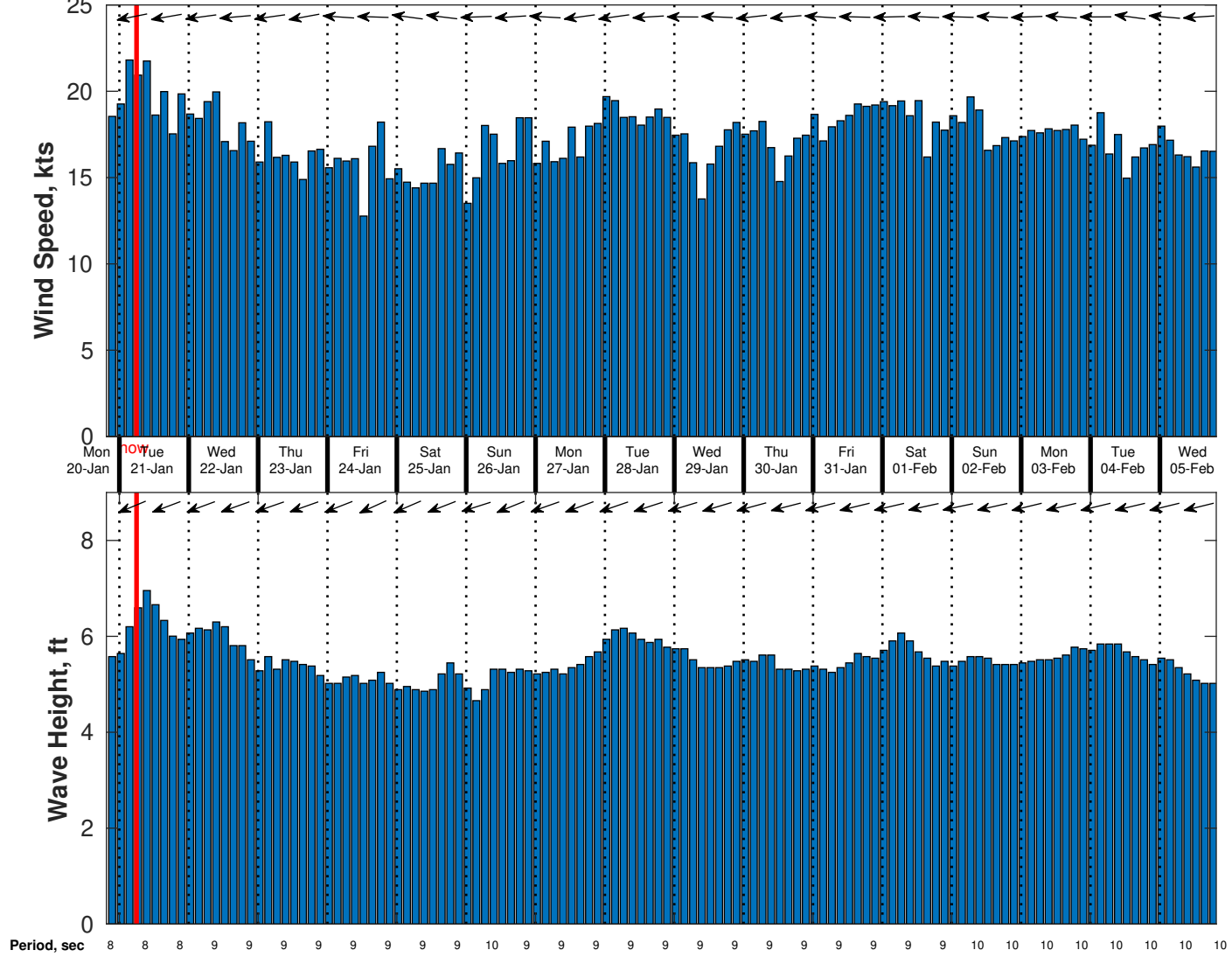
Wind & Wave Forecast for Geohira (Shell) Dragon from 20-Jan-2025 20:00:00 to 05-Feb-2025 20:00:00
