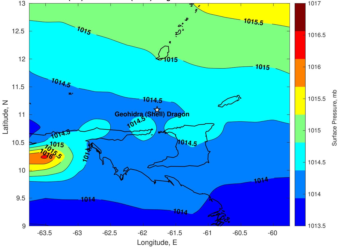
Surface Pressure (mb) for Geohidra (Shell) Dragon at 21-Jan-2025 00:00:00
