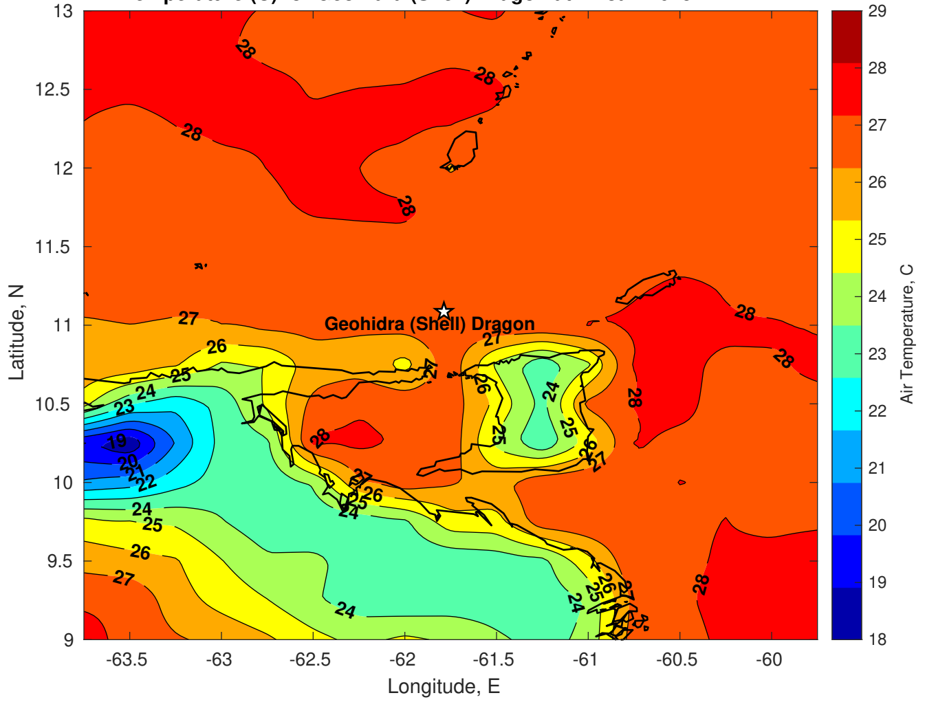
Air Temperature (C) for Geohidra (Shell) Dragon at 21-Jan-2025
