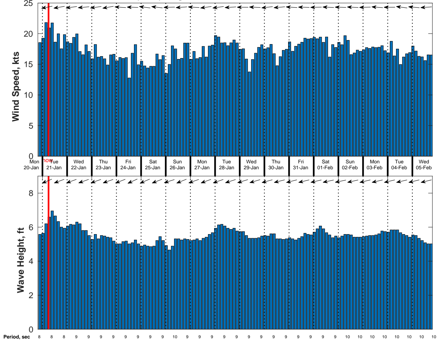
Wind & Wave Forecast for Geohdra (Shell) Dragon from 20-Jan-2025 20:00:00 to 05-Feb-2025 20:00:00
