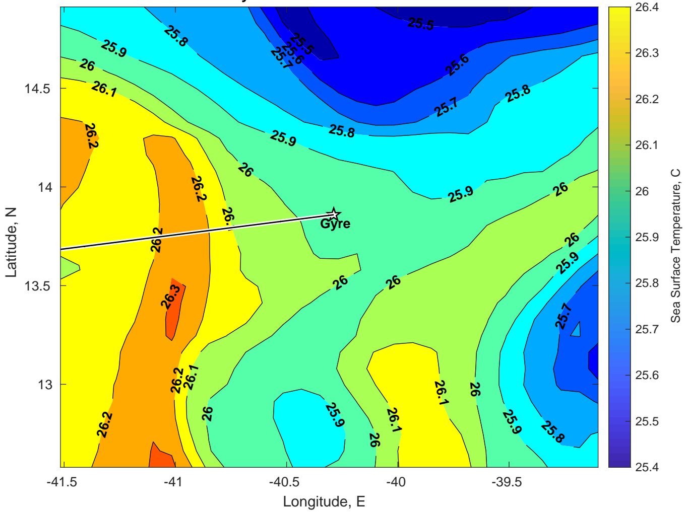
SST for Gyre at 20-Jan-2025 00:00:00
