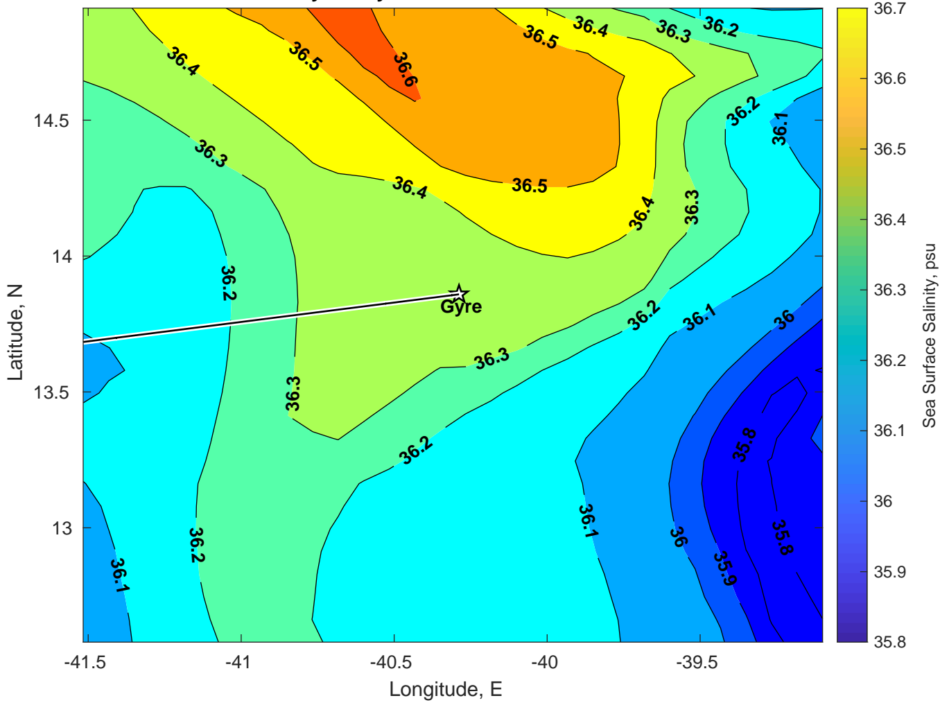
Surface Salinity for Gyre at 20-Jan-2025 00:00:00
